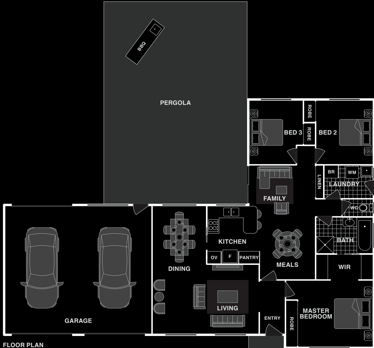
FLOOR PLAN
