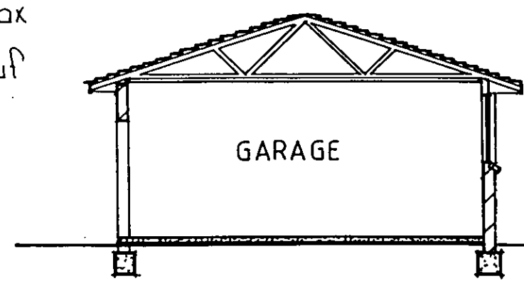
SECTION
