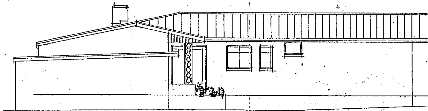
SIDE ELEVATION
