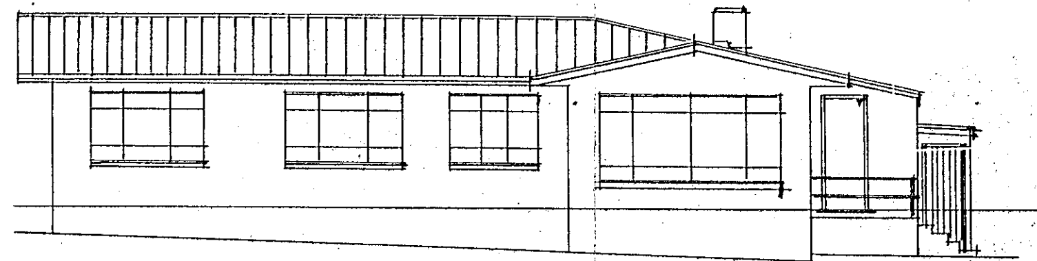
SIDE ELEVATION
