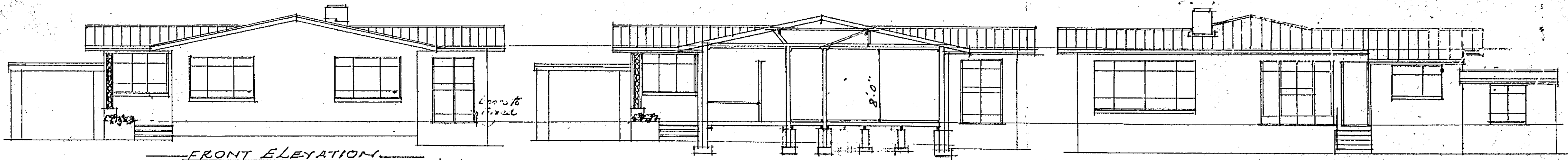
FRONT ELEVATION
