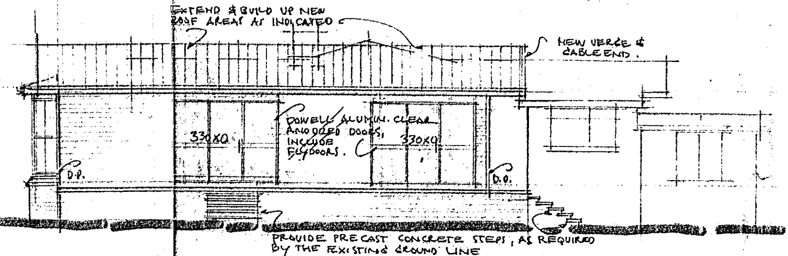
WEST ELEVATION
