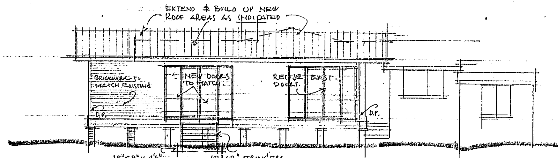
WEST ELEVATION
