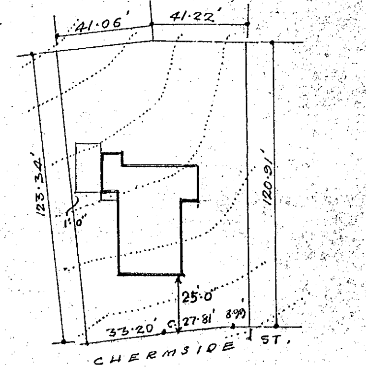
BLOCK PLAN 40' = 1"
