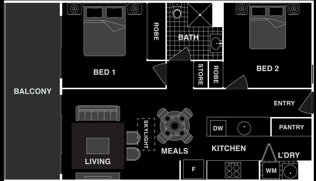
FLOOR PLAN
