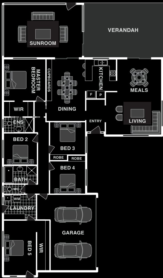
FLOOR PLAN
