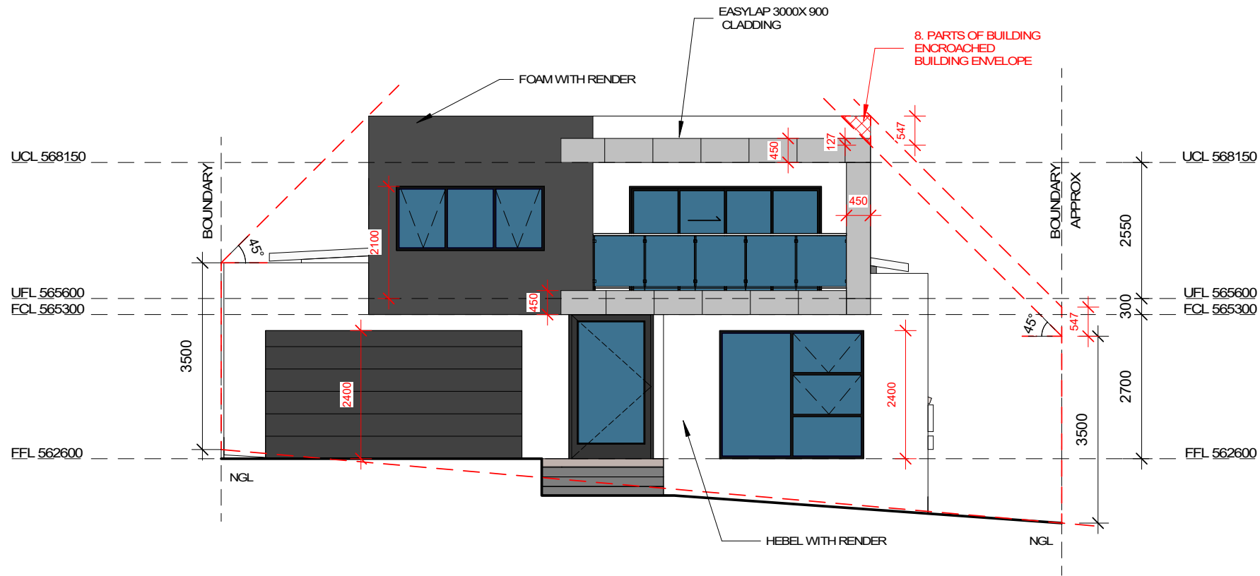
1 ELEVATION 1 : 100 South Elevation
