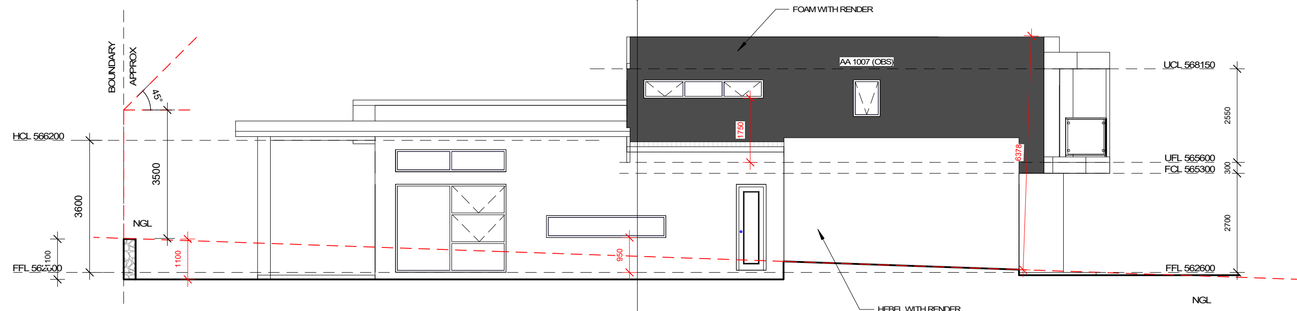
2 ELEVATION 1 : 100 West Elevation
