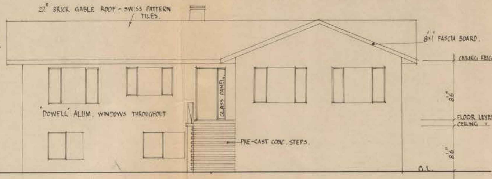
EAST ELEV.
