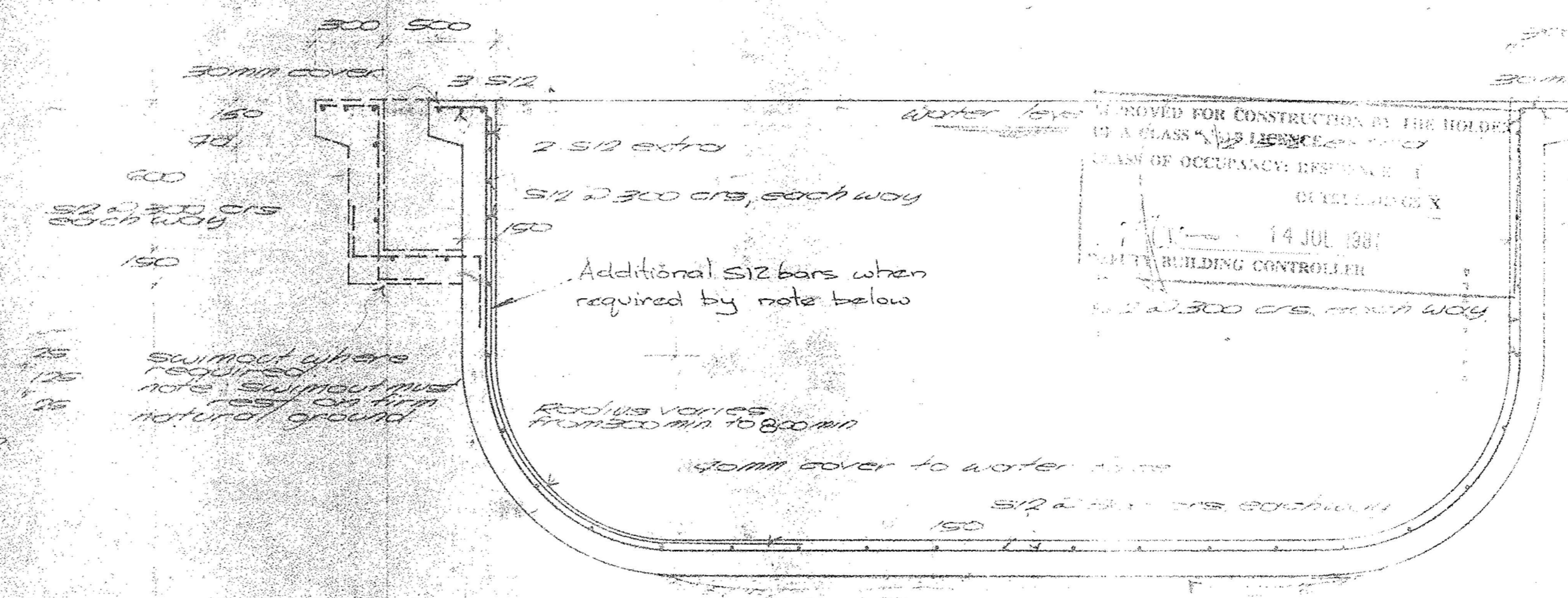
TYPICAL SECTION AT STEPS 1:20
