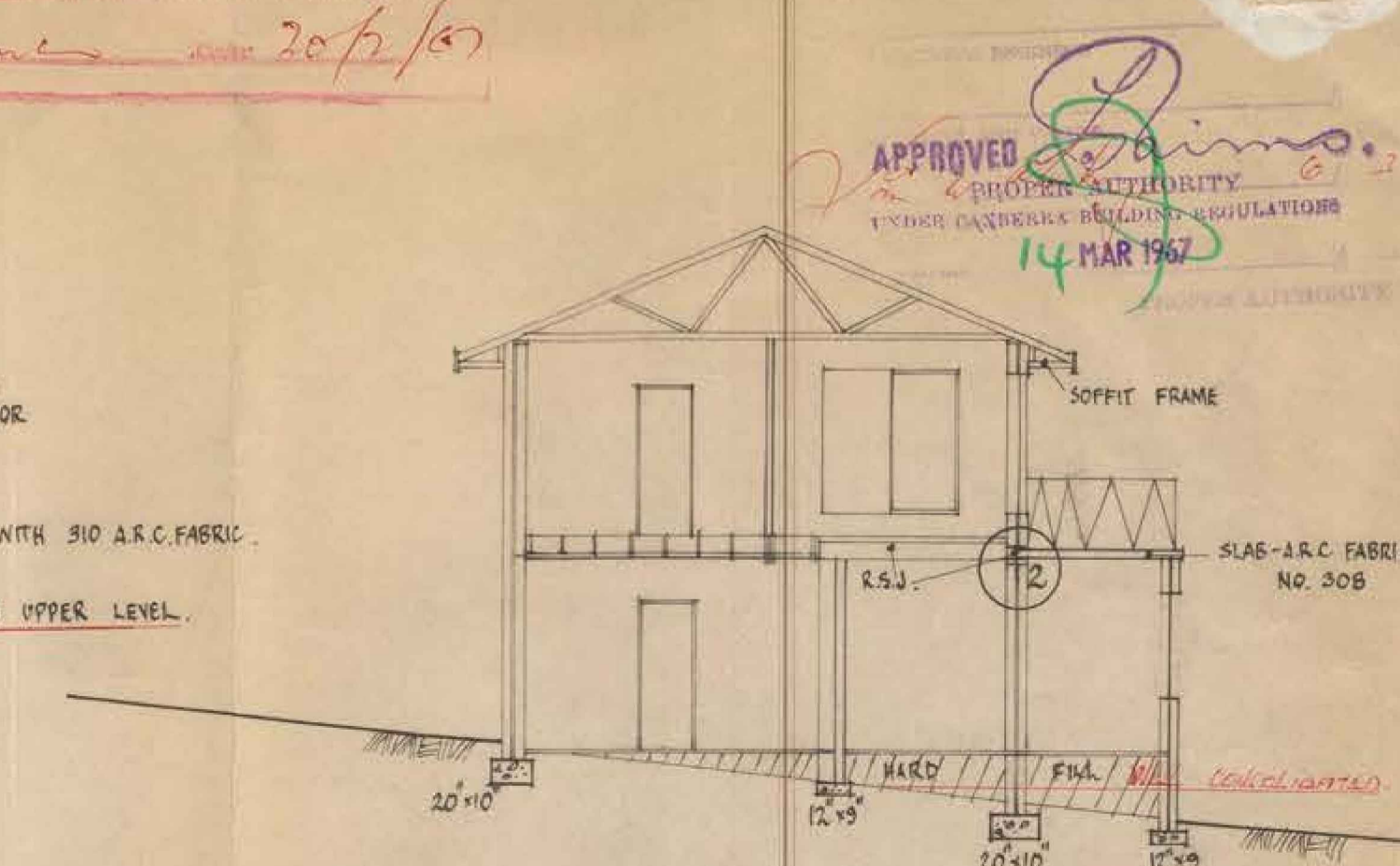
SECT. A.A.
