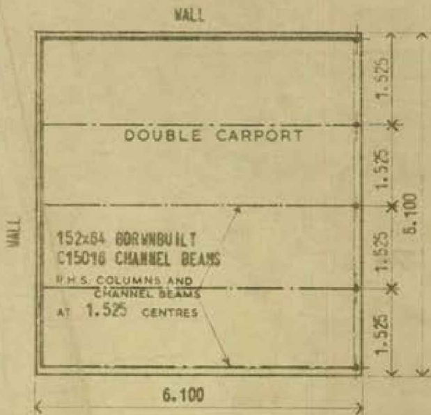
PLAN (TYPICAL) SCALE: 1 : 100
