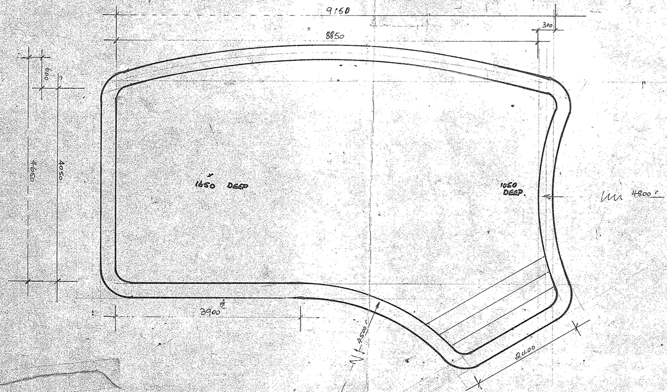
PLAN POOL
