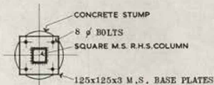
COLUMN PLAN
