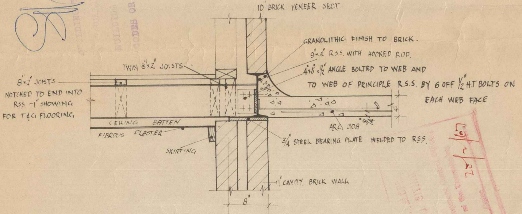
DETAIL 2
