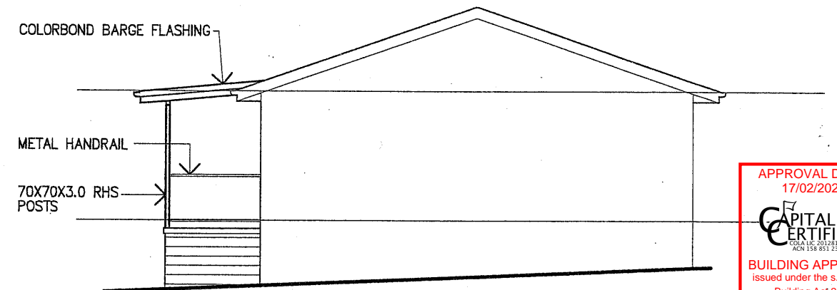
NORTH ELEVATION 1:100
