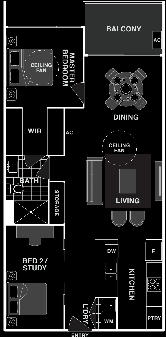
FLOOR PLAN
