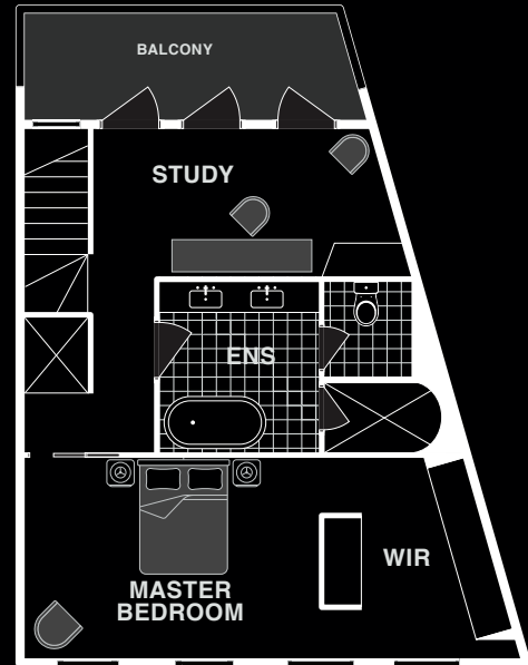
SECOND LEVEL
