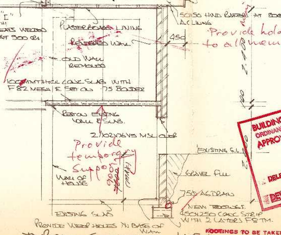
TYPICAL SECTION 1:50
