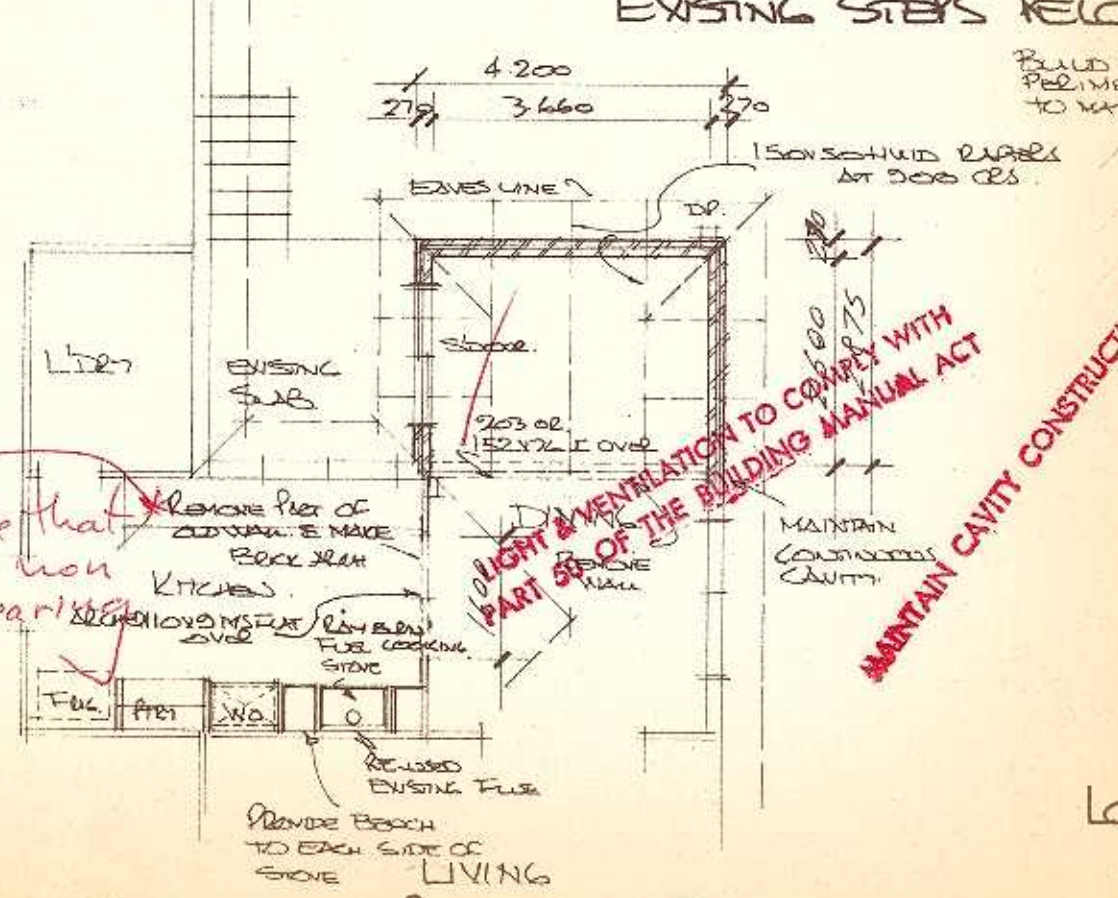
GENERAL PLAN 1:100
