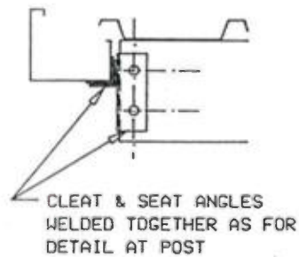
DETAIL OF PURLIN NOT AT A POST SCALE 1:100
