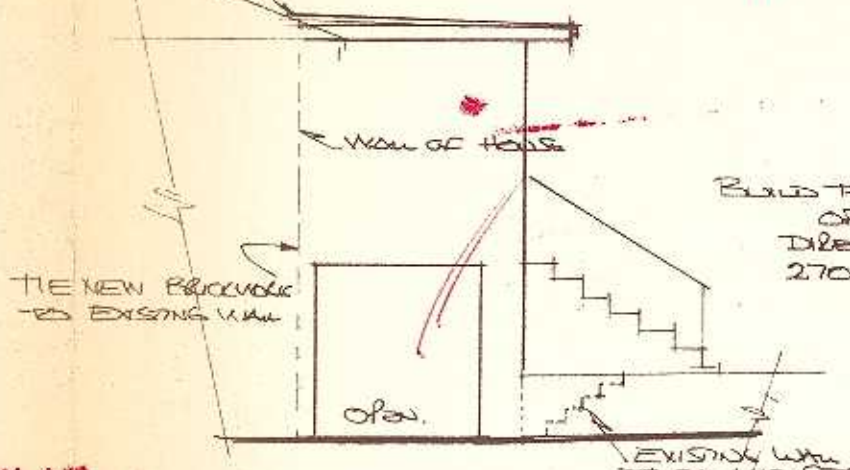
SIDE ELEVATION 1:100
