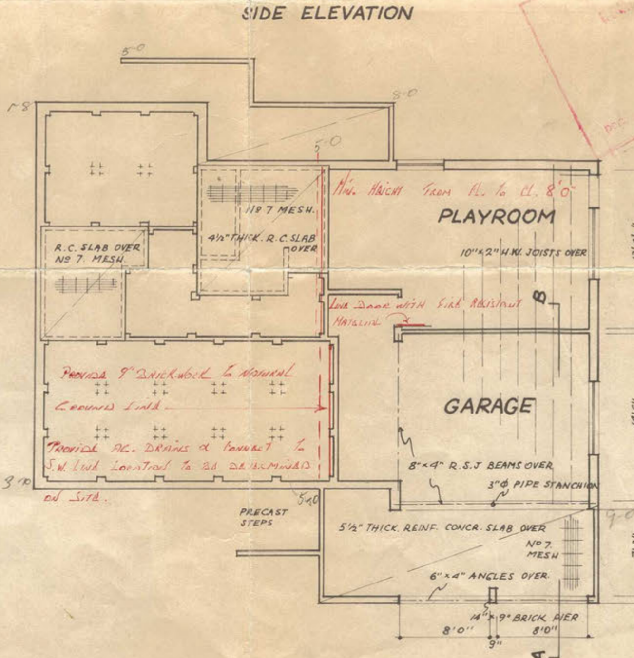
BASEMENT PLAN
