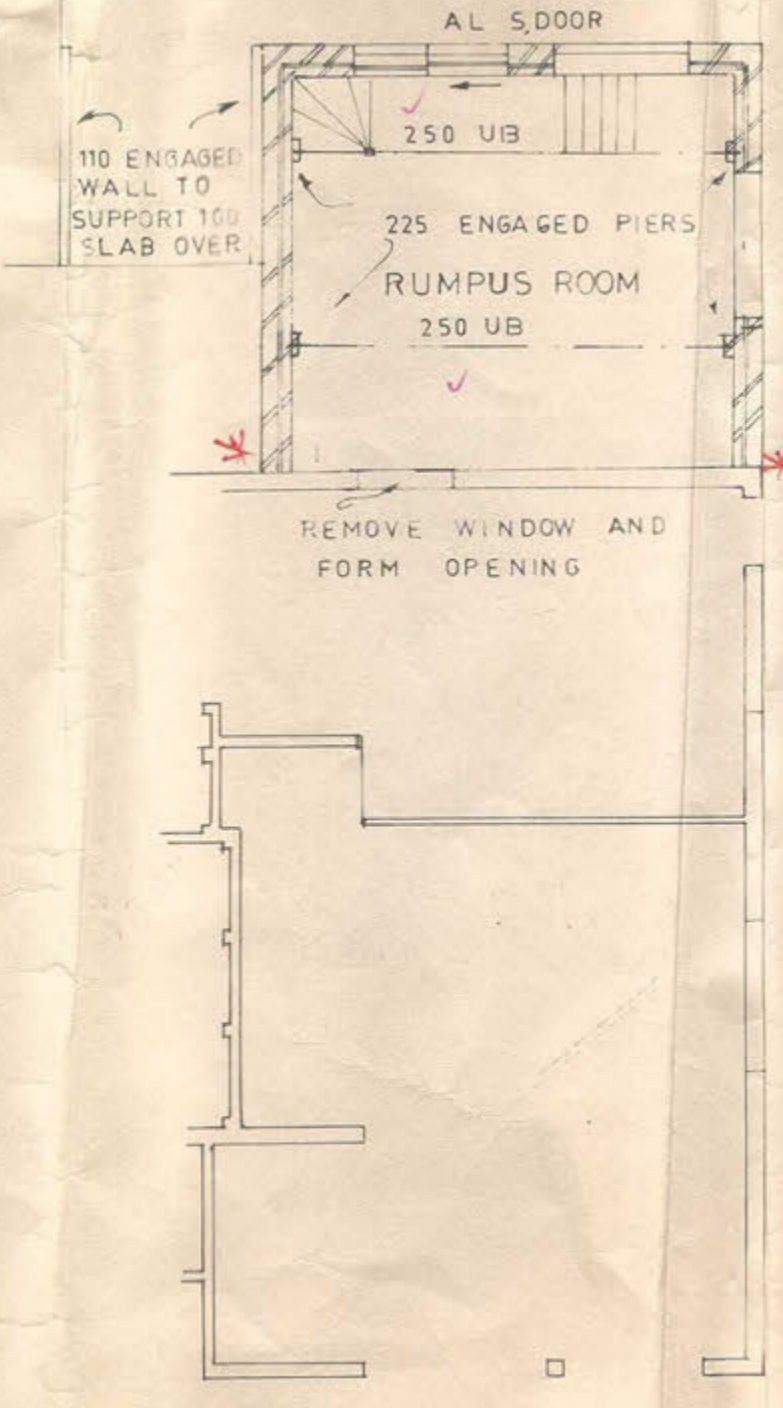
PLAN LOWER LEVEL
