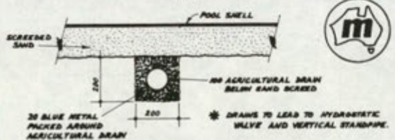
TYPICAL AGRICULTURAL DRAIN
