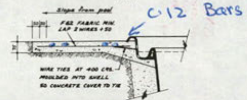
REINFORCEMENT & COPING DETAIL
