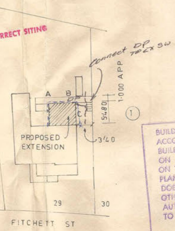
SITE PLAN
