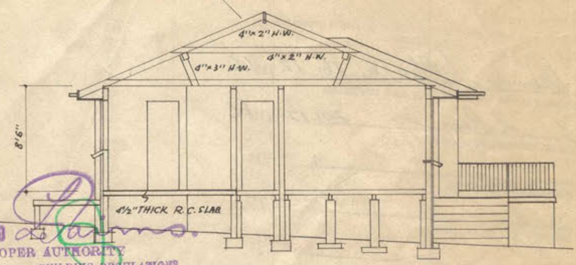
SECTION X-X
