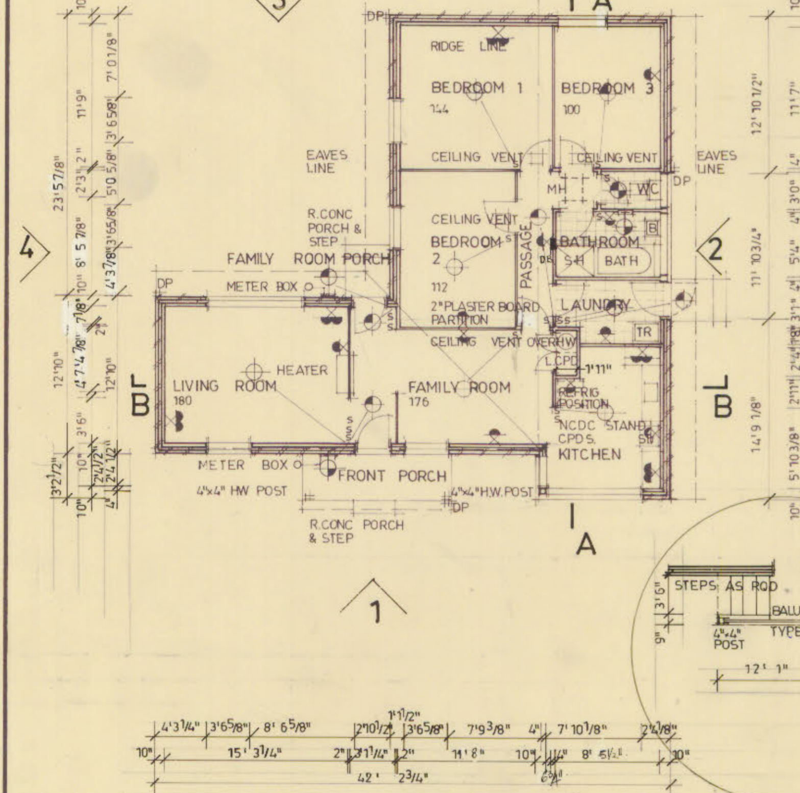
FLOOR PLAN
