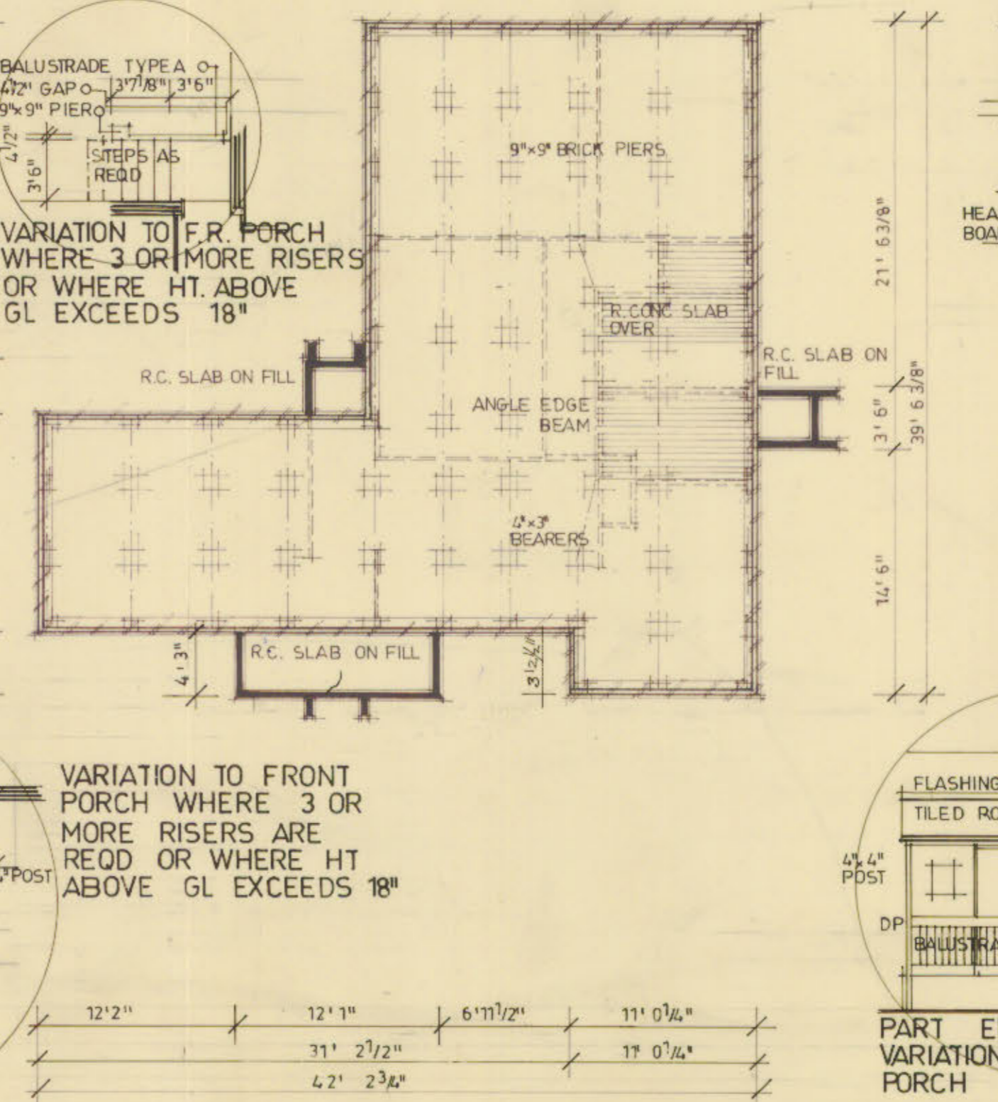
FOUNDATION PLAN
