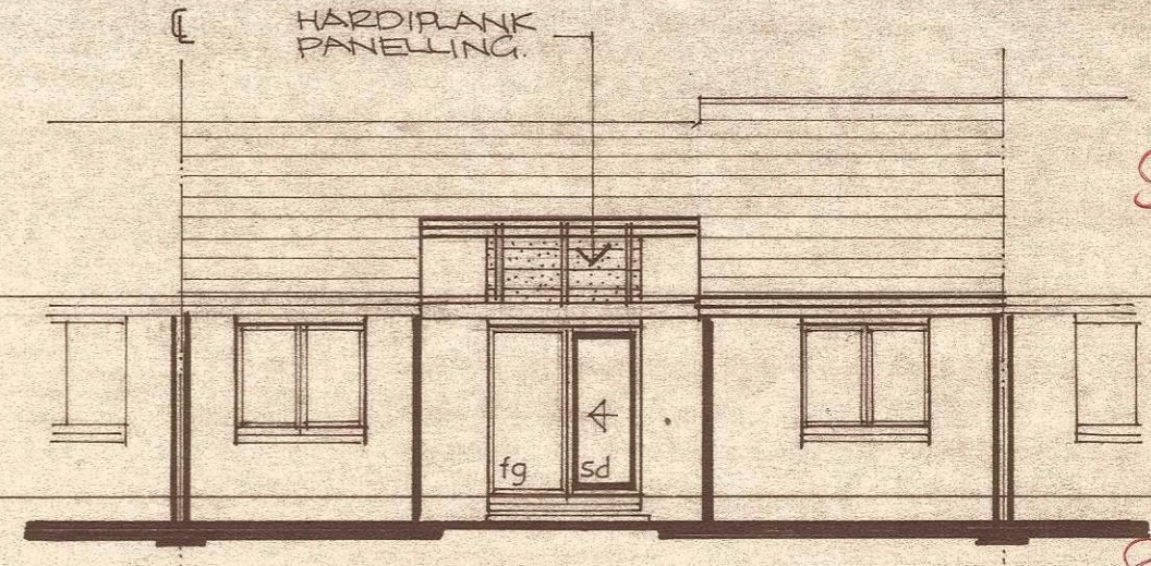
REAR ELEVATION 1:100
