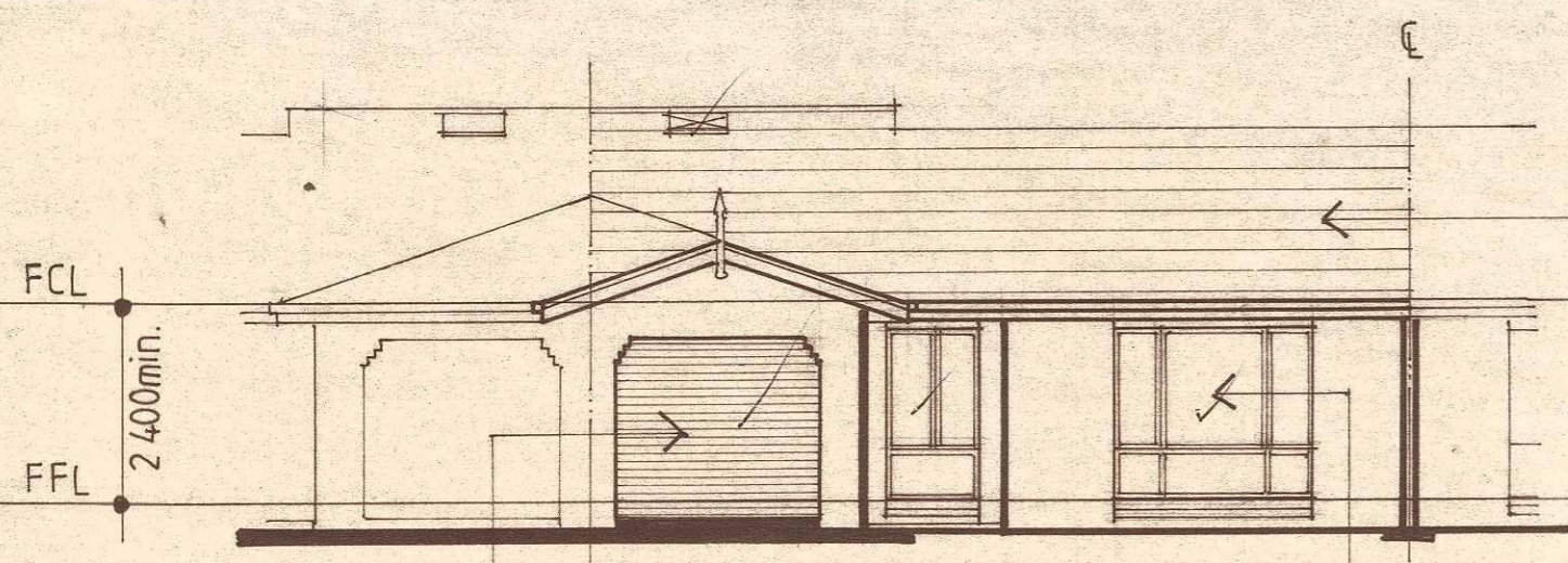
FRONT ELEVATION 1:100
