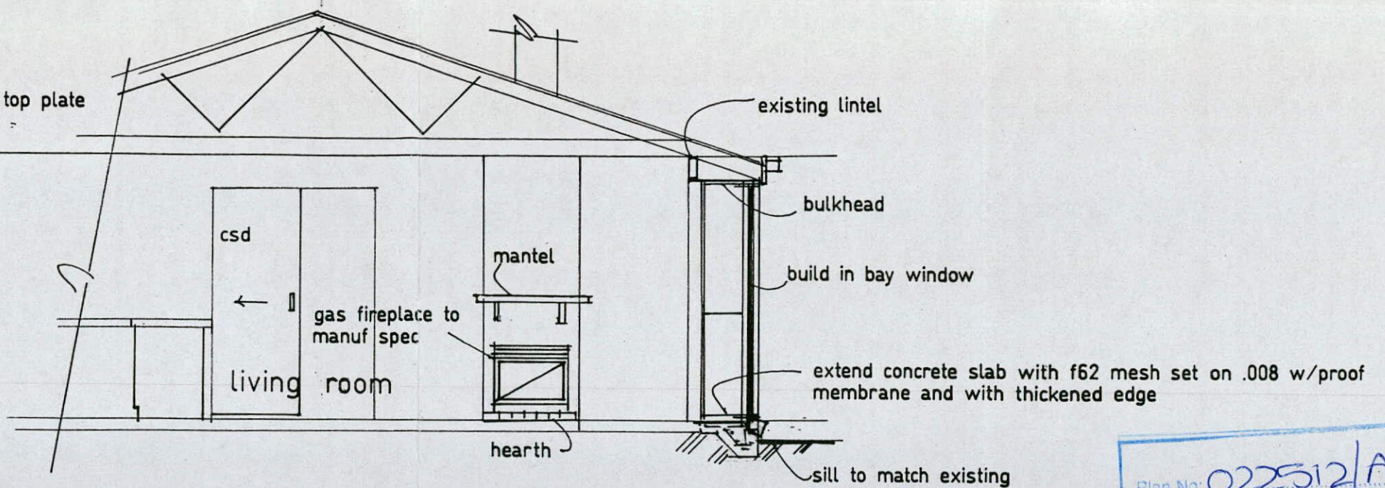
LIVING SECTION 1.50
