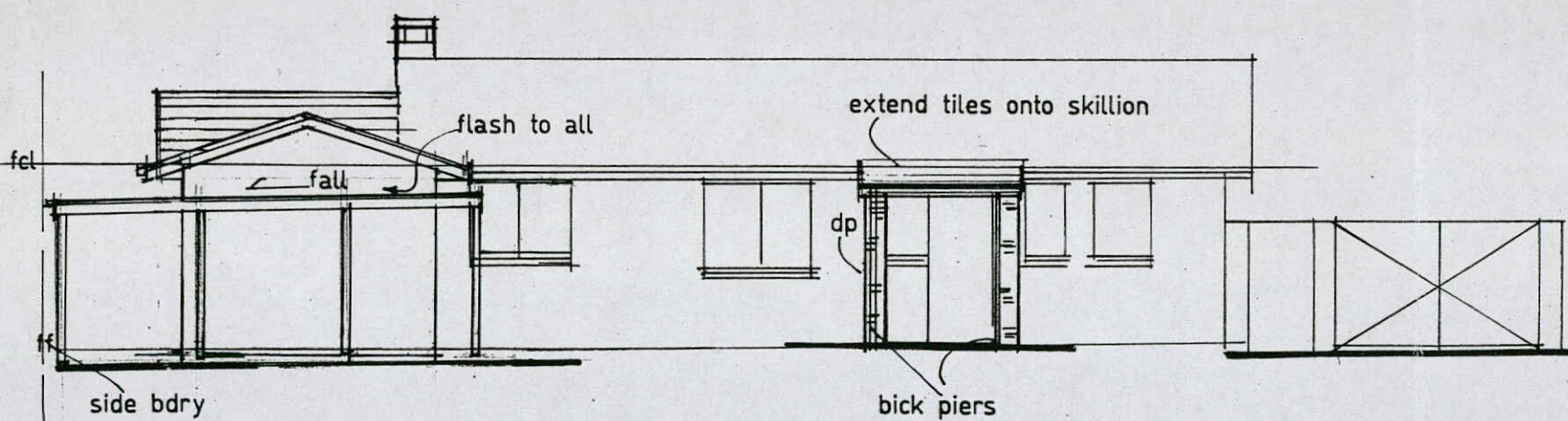
REAR ELEVATION 1.100
