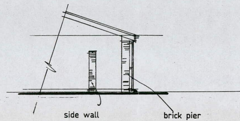
SIDE ELEVATION 1.100
