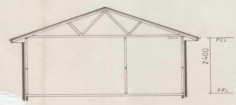
Section 1:100
