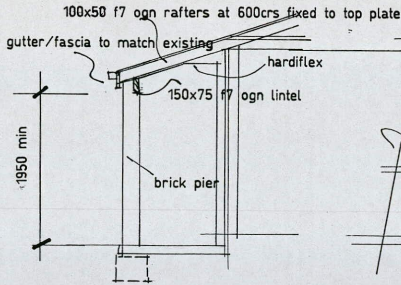
SKILLION SECTION 1.50
