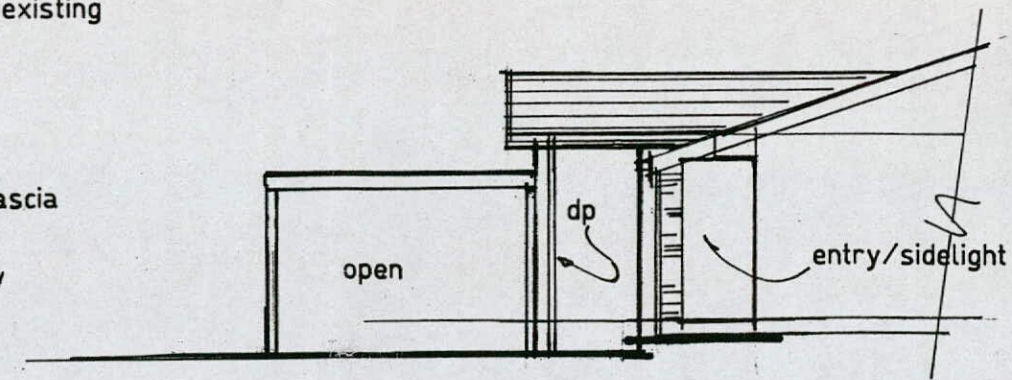
SIDE ELEVATION 1.100
