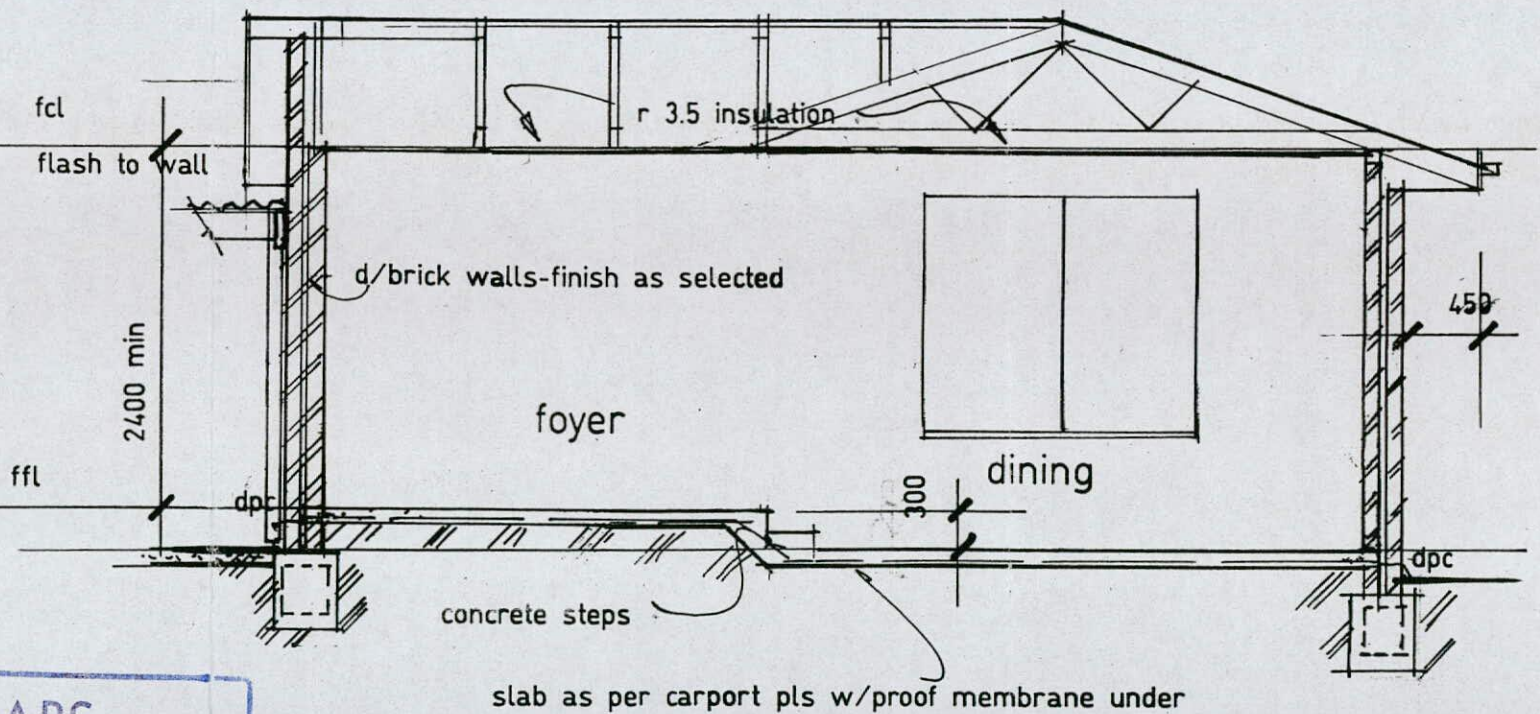
CROSS SECTION 1.50
