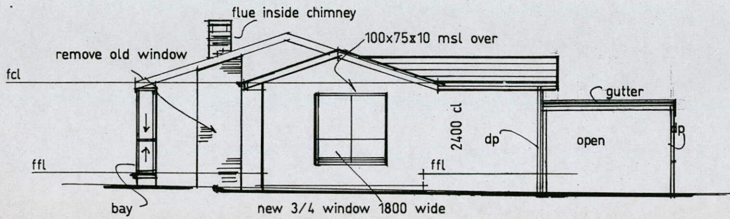
SIDE ELEVATION 1.100
