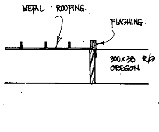
detail b-b 1:20
