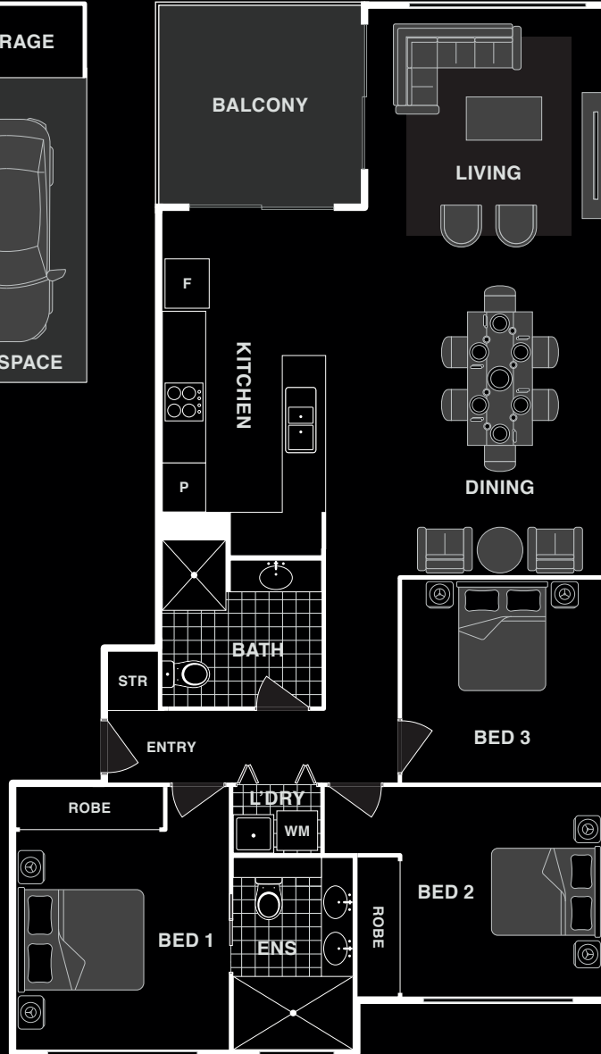
FLOOR PLAN
