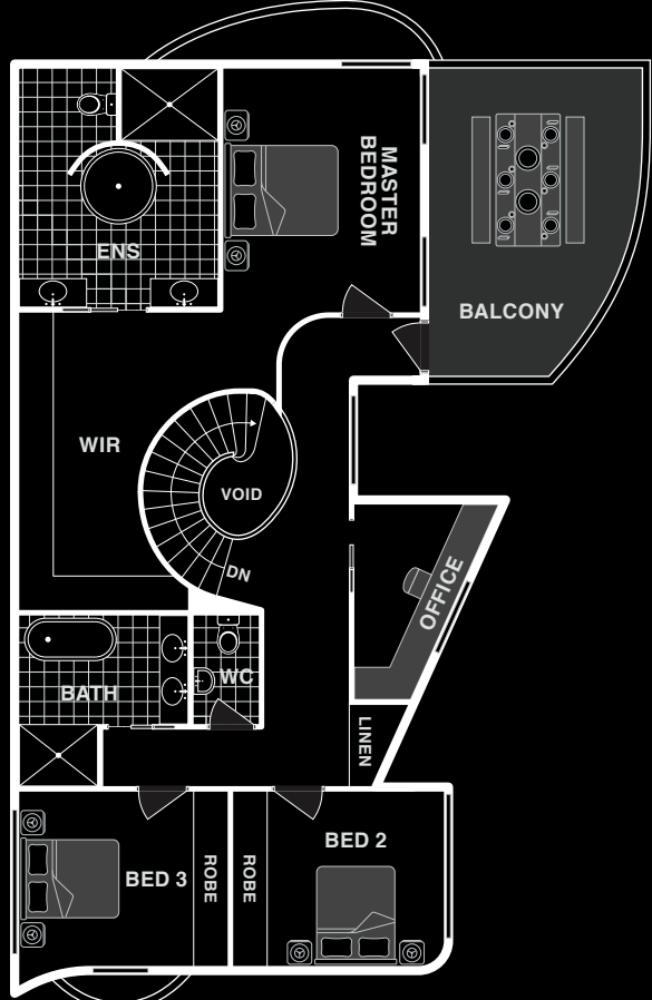
UPPER LEVEL
