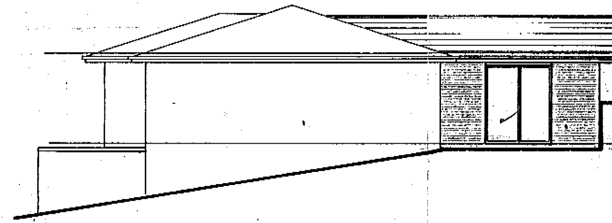
ELEVATION 3.
