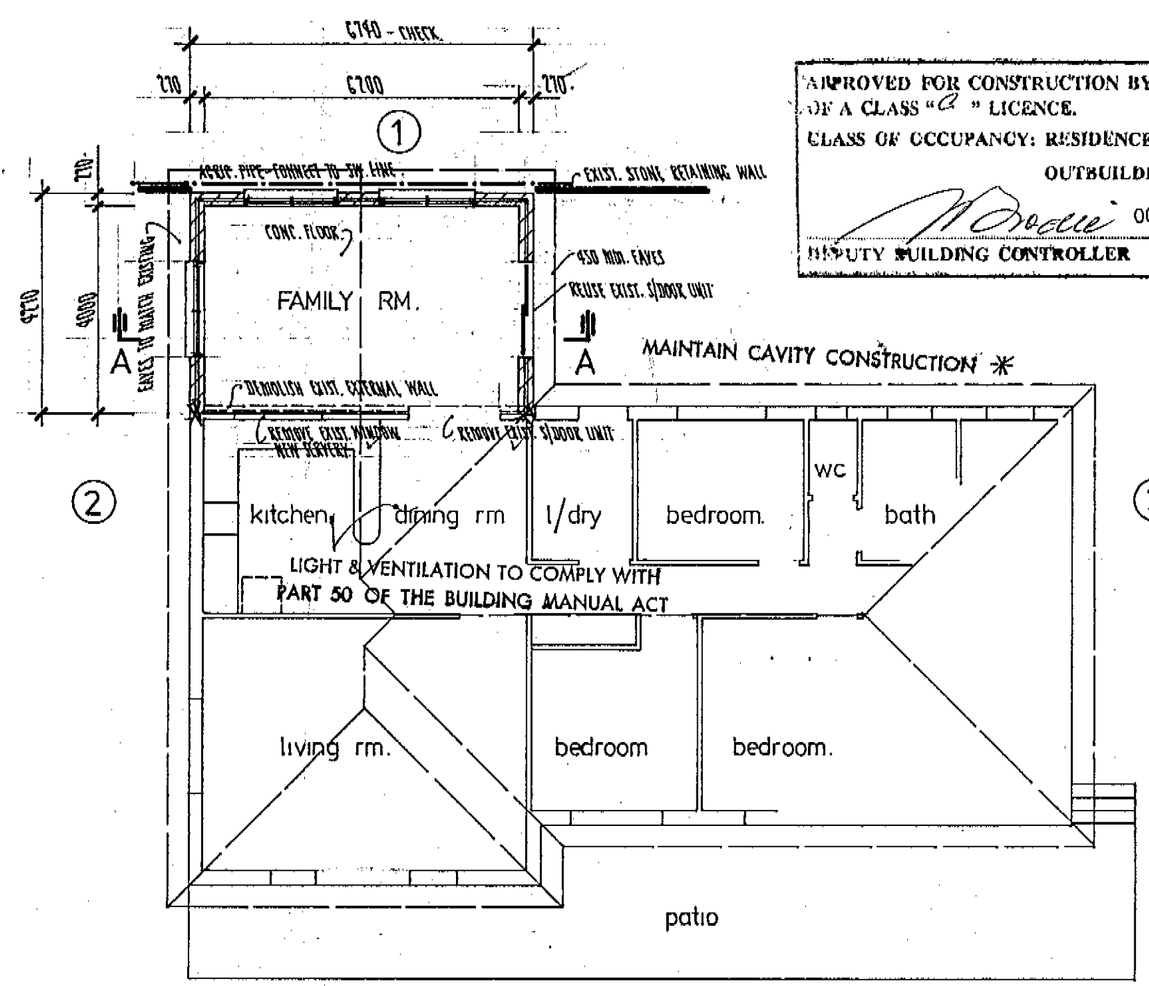
FLOOR PLAN.
