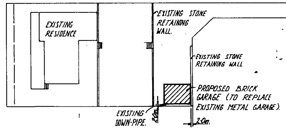
SITE PLAN NO PART OF THE STRUCTURE/FOOTINGS TO ENCROACH THE BOUNDARY SCALE - 1:500
