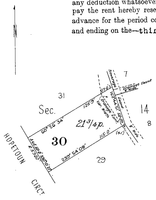
Scale: 60 feet to an inch
