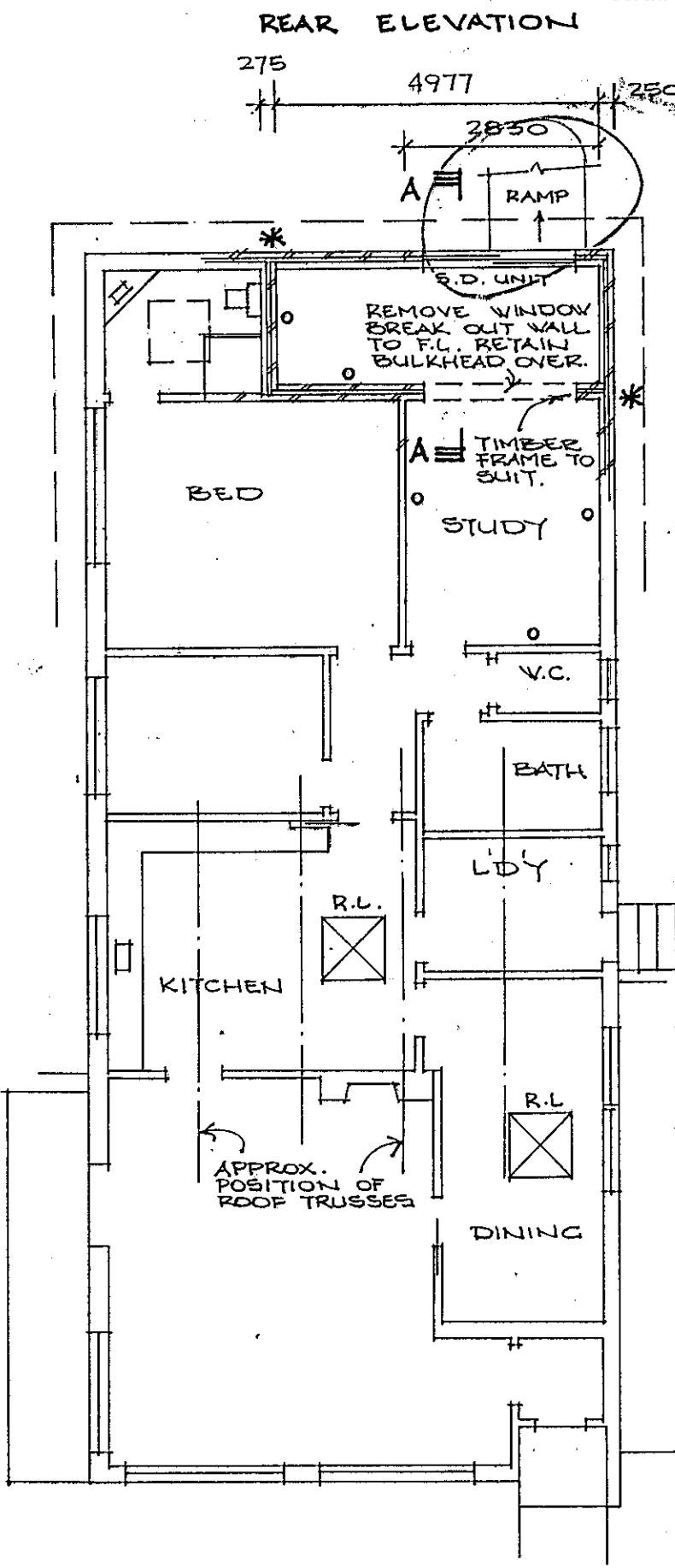
FLOOR PLAN
