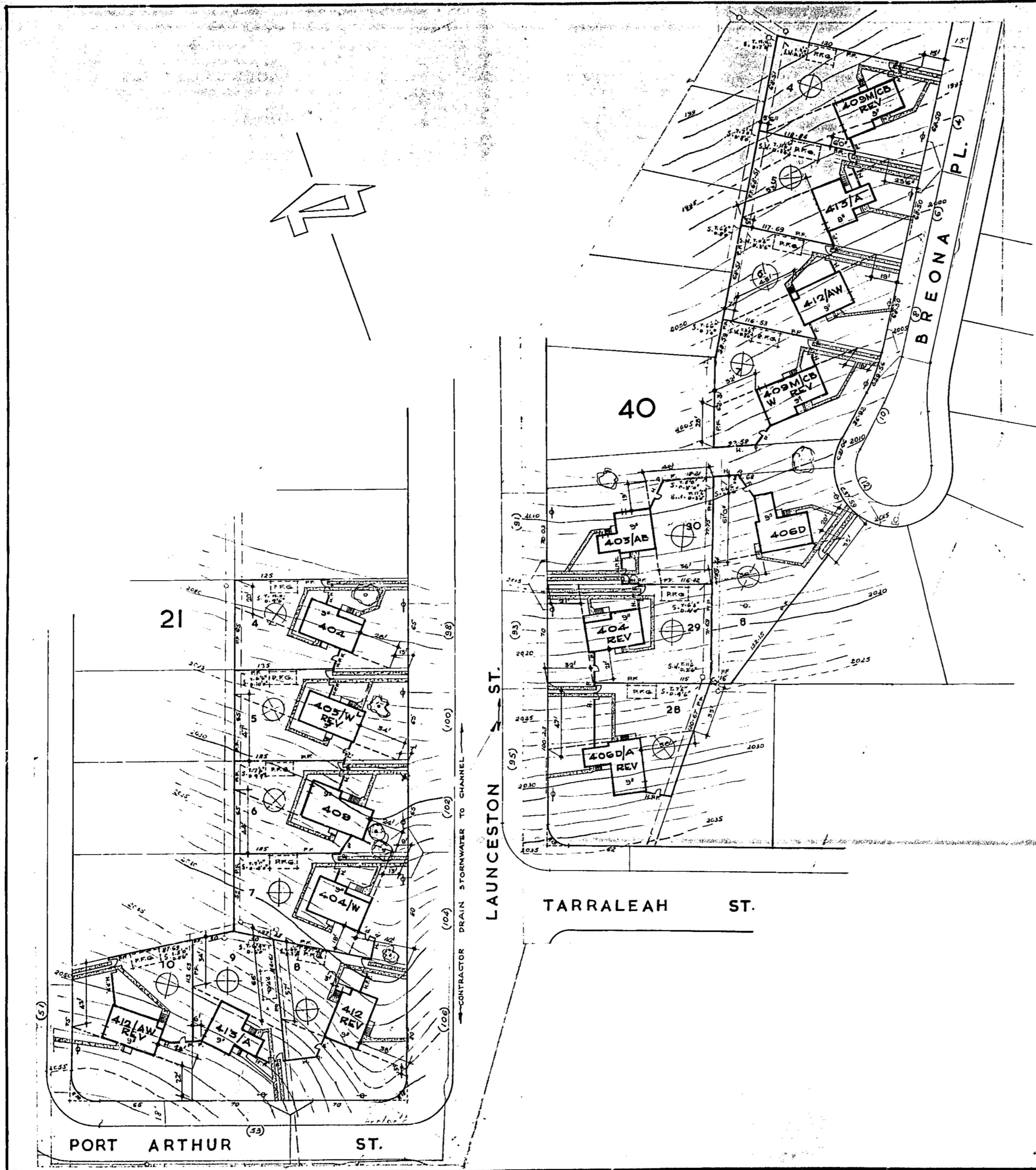
LOCATION PLAN
