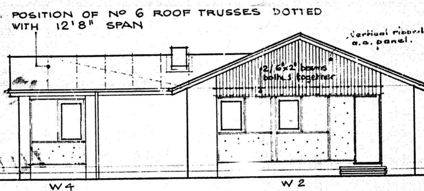
ELEVATION ③
