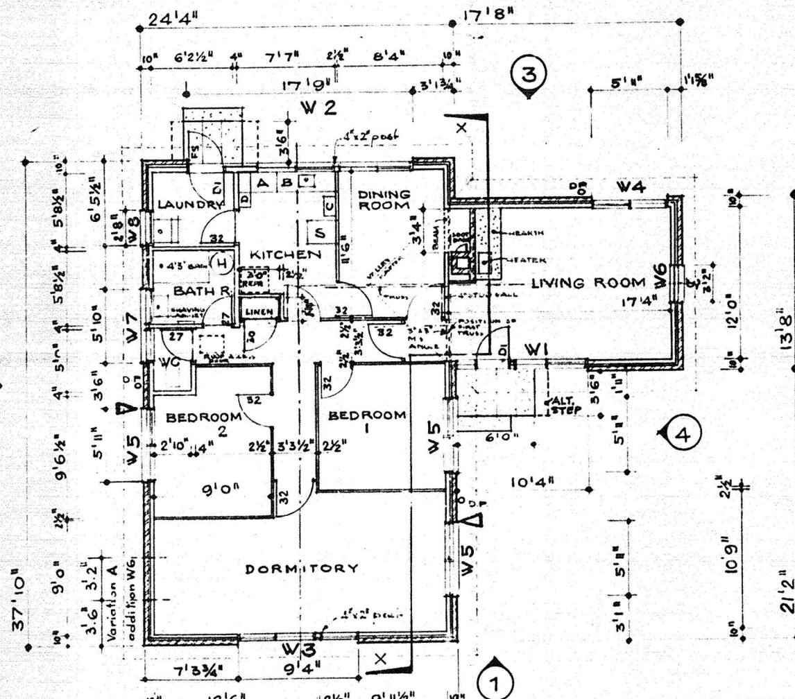
PLAN
