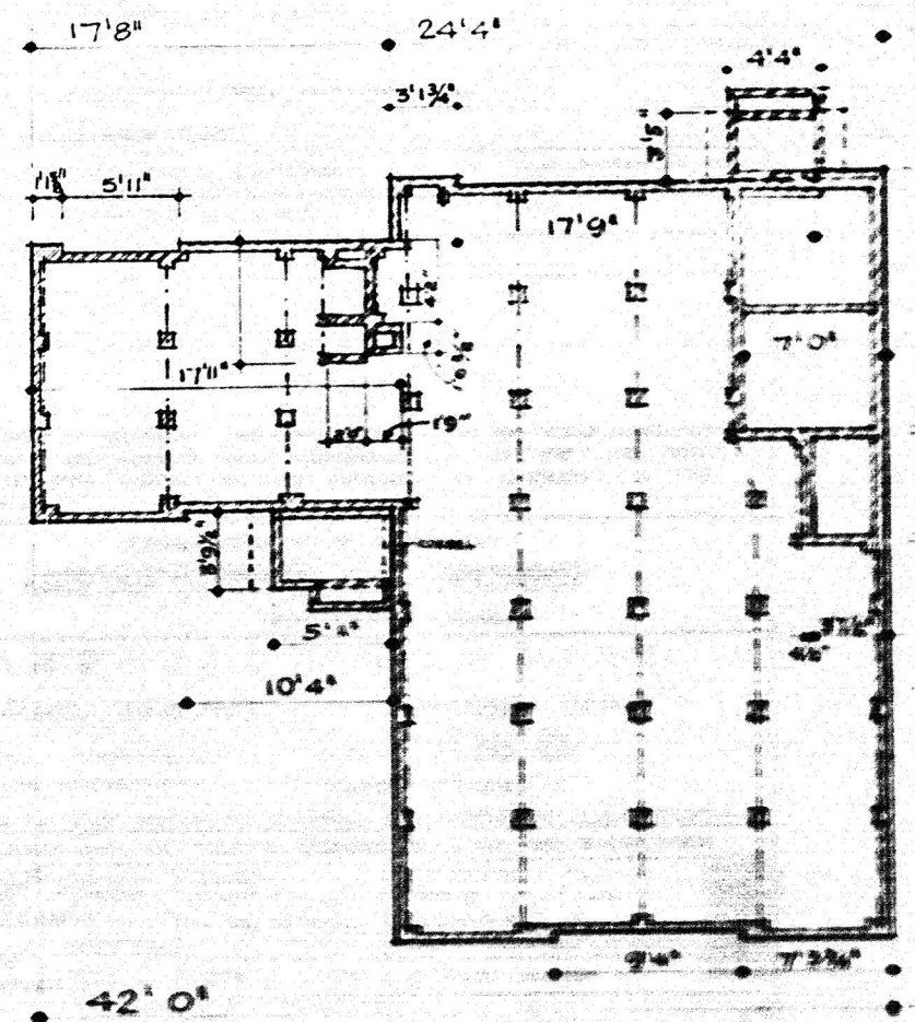
REVERSED PLAN OF FOOTING WALLS
