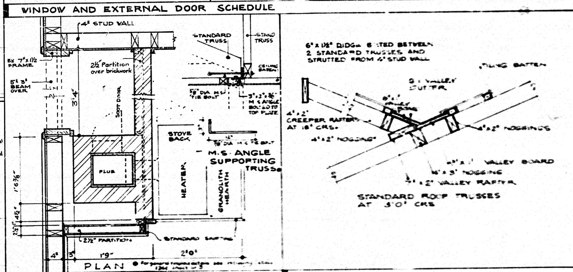
CHIMNEY AND WALL RECESS SCALE 1/4" TO 1'0"
