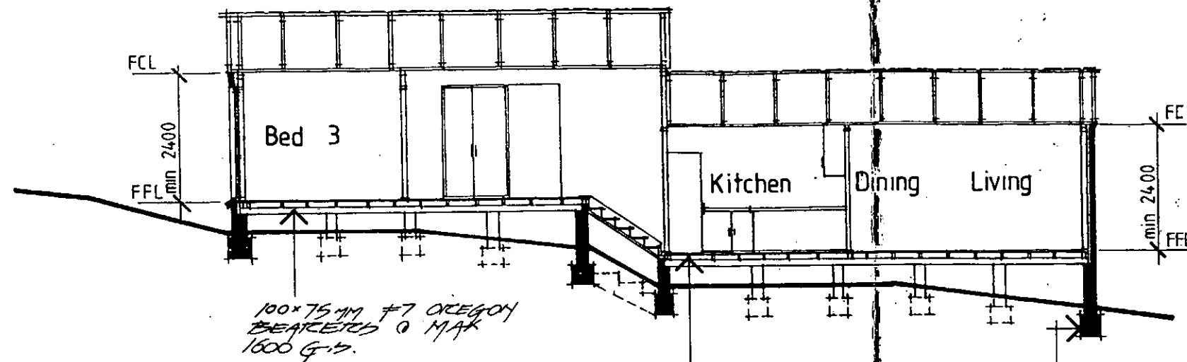
SECTION - B 1:100
