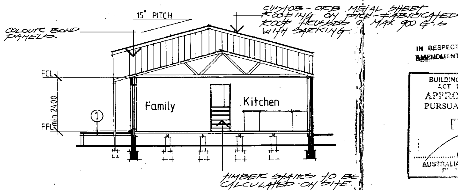
SECTION A 1:100
