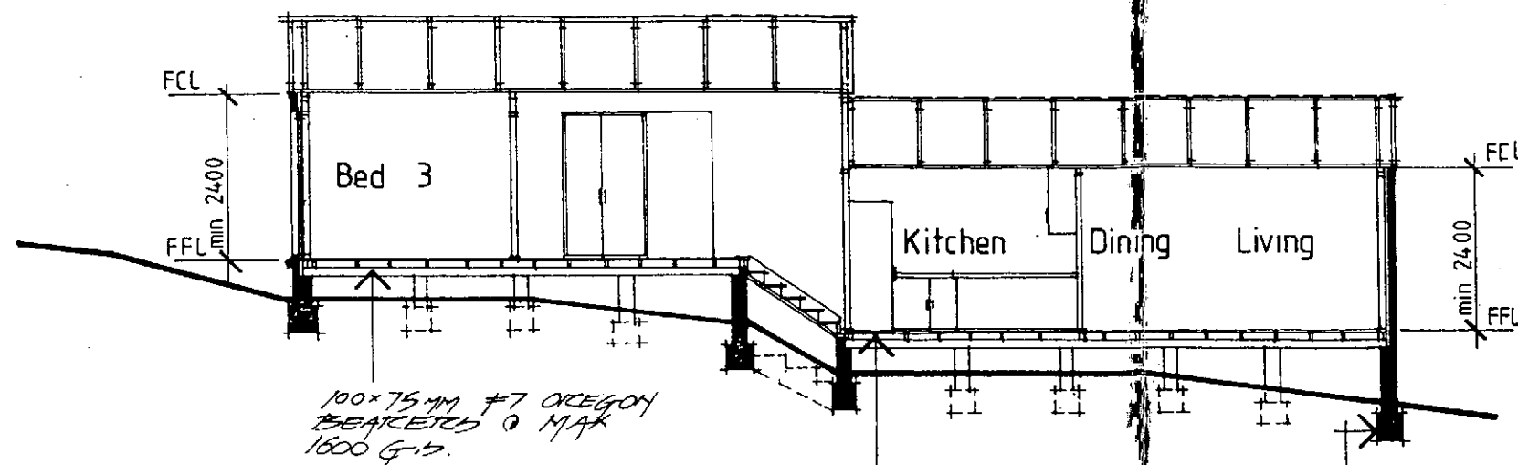
SECTION-B 1:100
