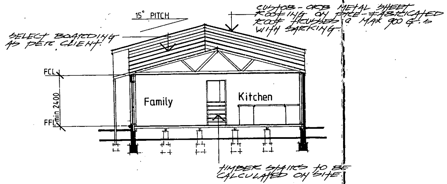
SECTION A 1:100
