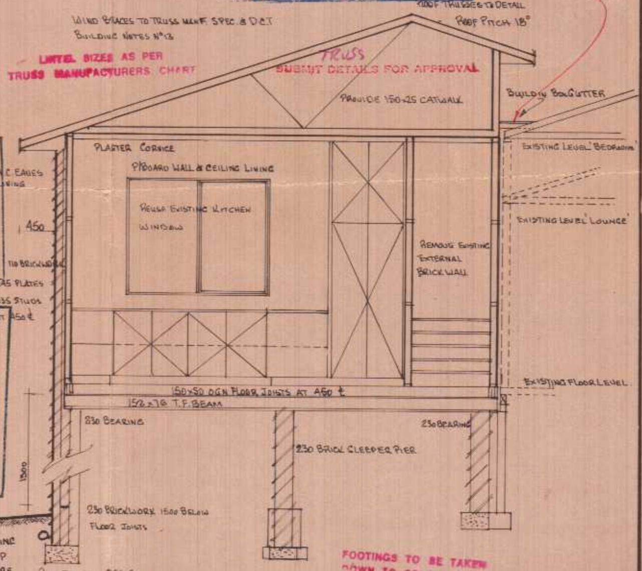
SECTIONAL ELEVATION
