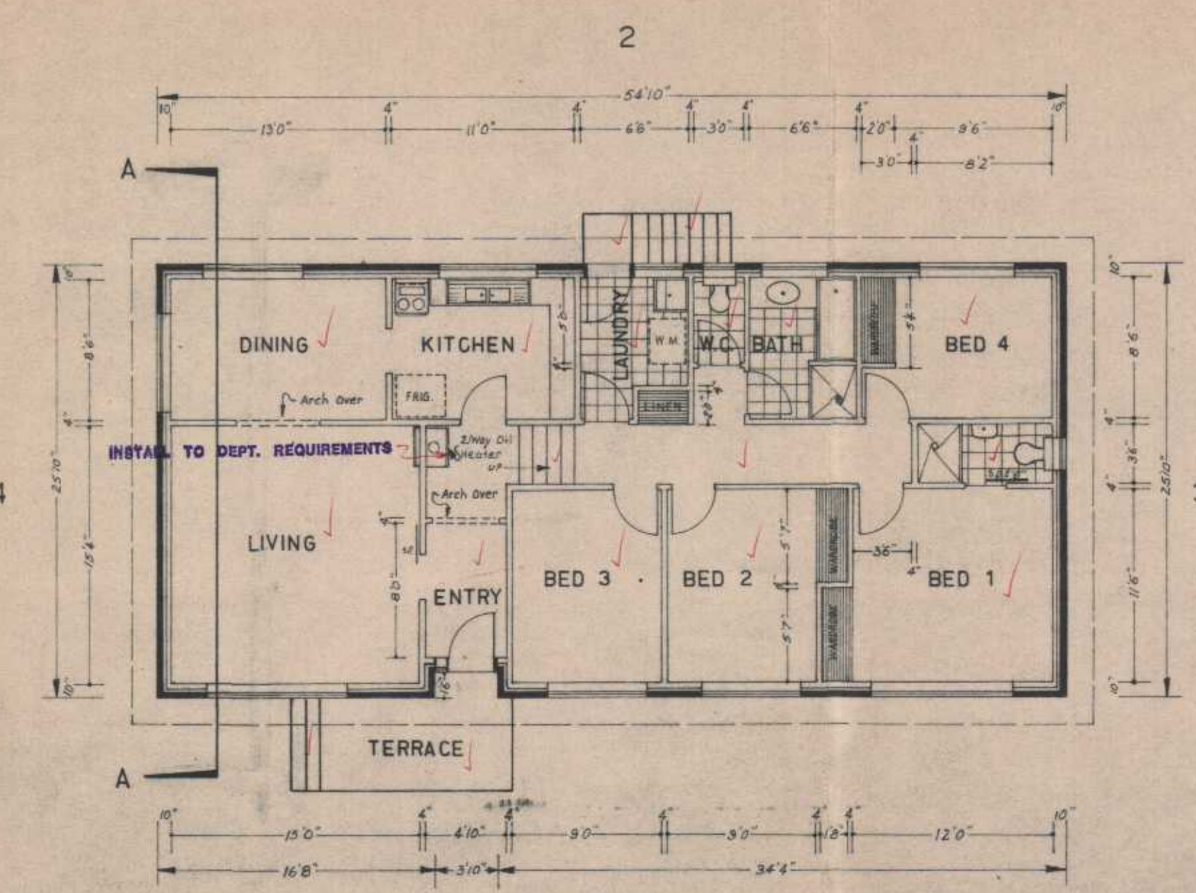
FLOOR PLAN
