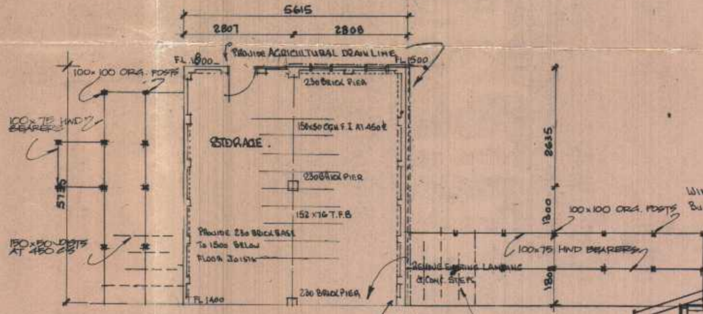
FOUNDATION PLAN
