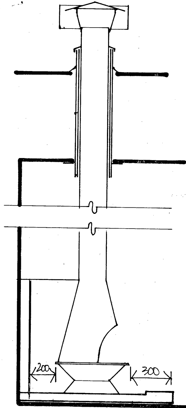
TYPICAL SECTION
