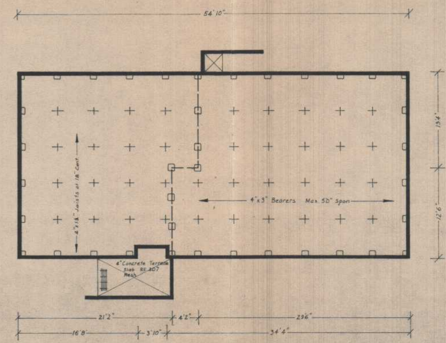
FOOTING PLAN
