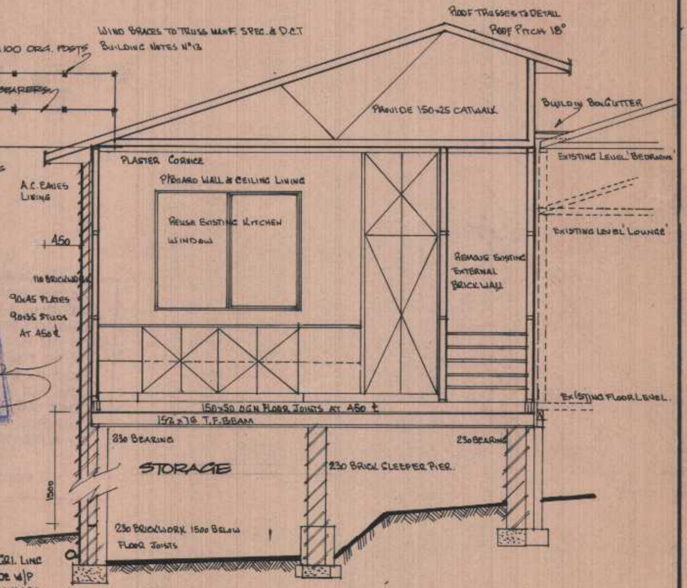
SECTIONAL ELEVATION
