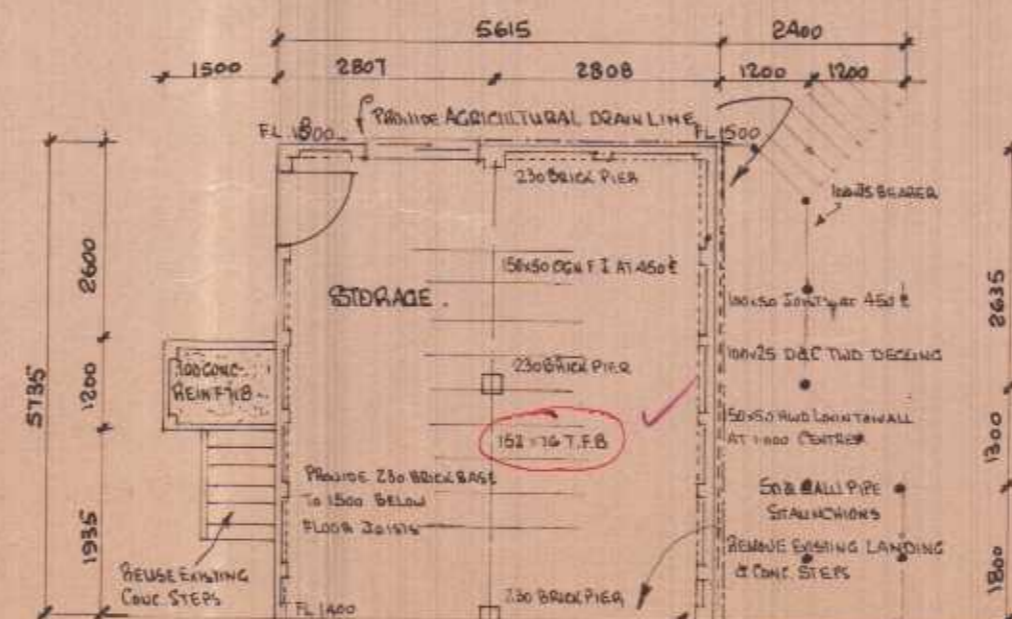
FOUNDATION PLAN
