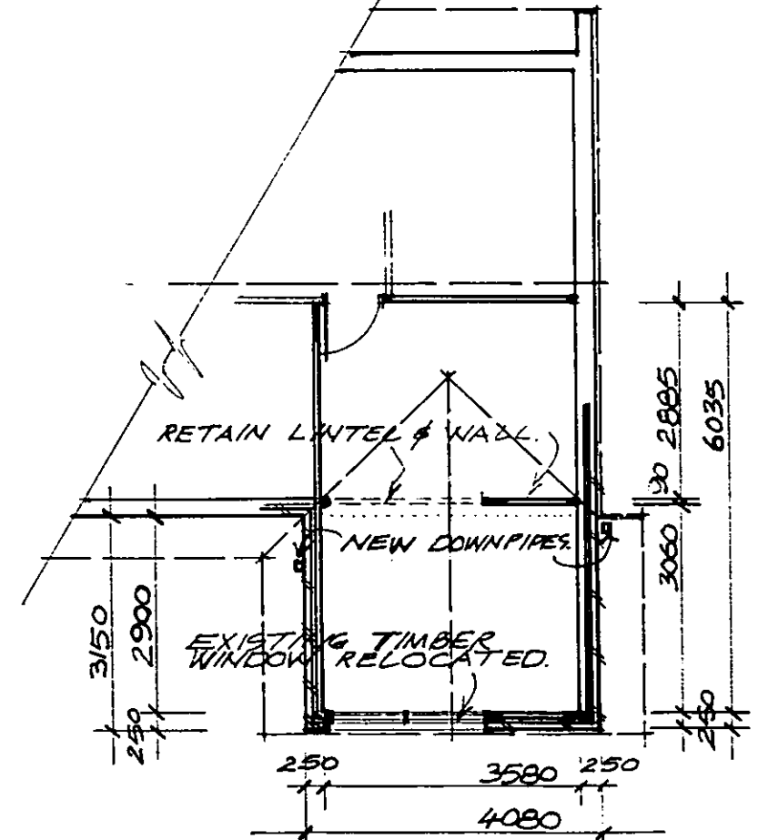
plan - proposed bedroom extension. scale 1:100
