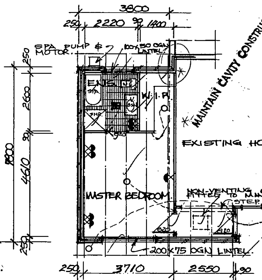
PLAN PROPOSED ADDITIONS SCALE 1:100 AREA 35.09 m 2
