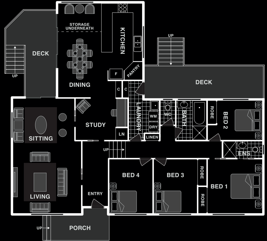
FLOOR PLAN
