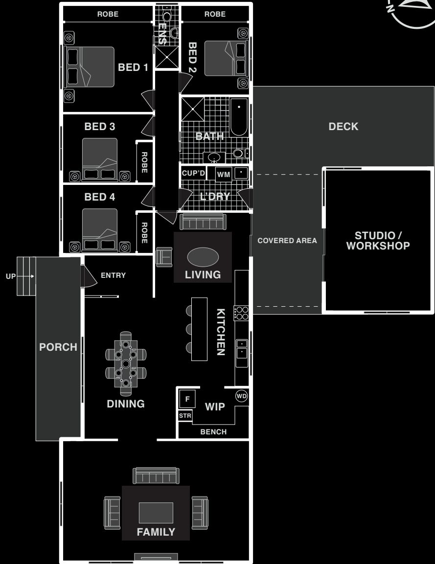
FLOOR PLAN
