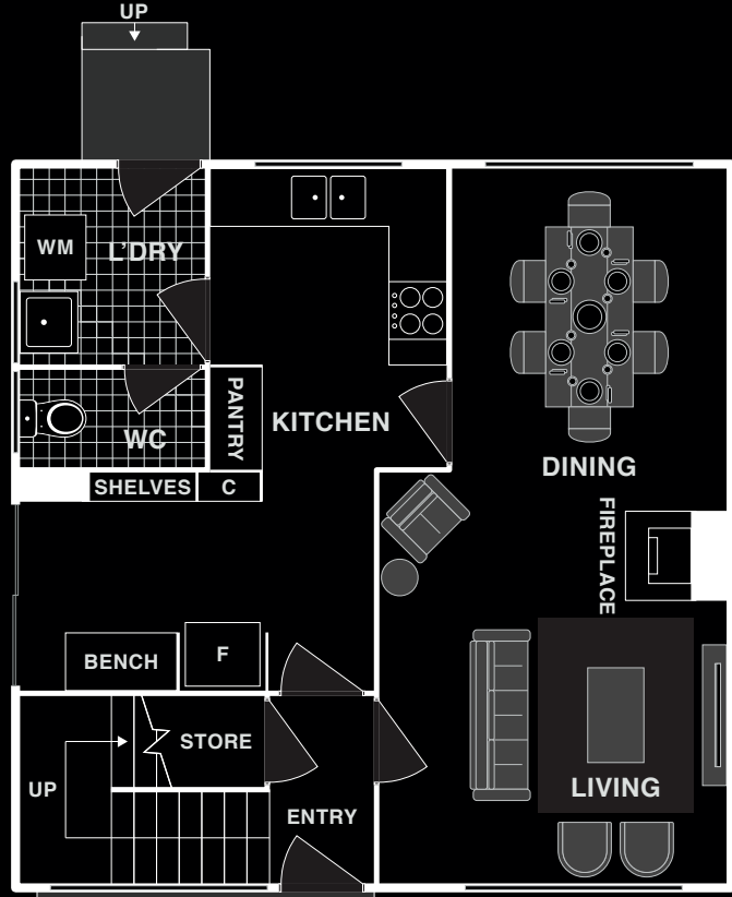
GROUND LEVEL
