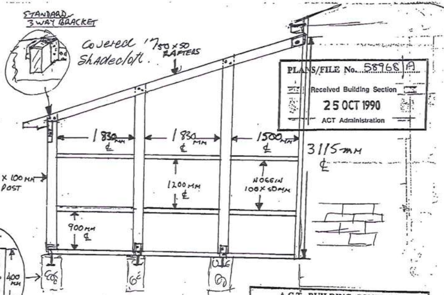
RIGHT HAND ELEVATION
