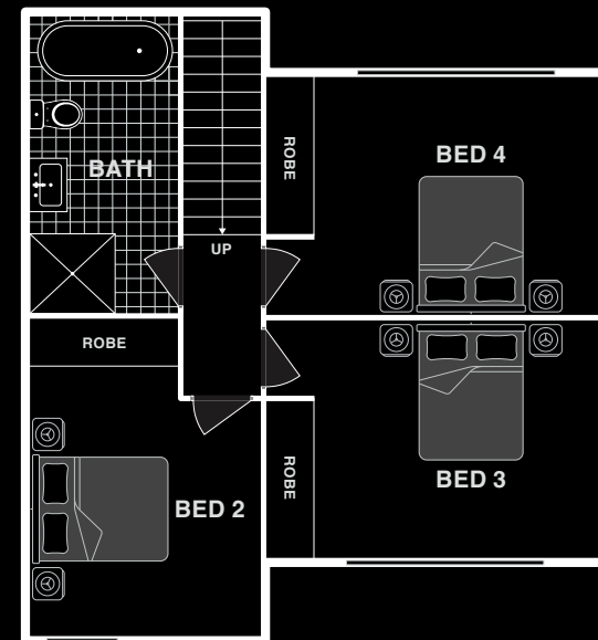
UPPER LEVEL
