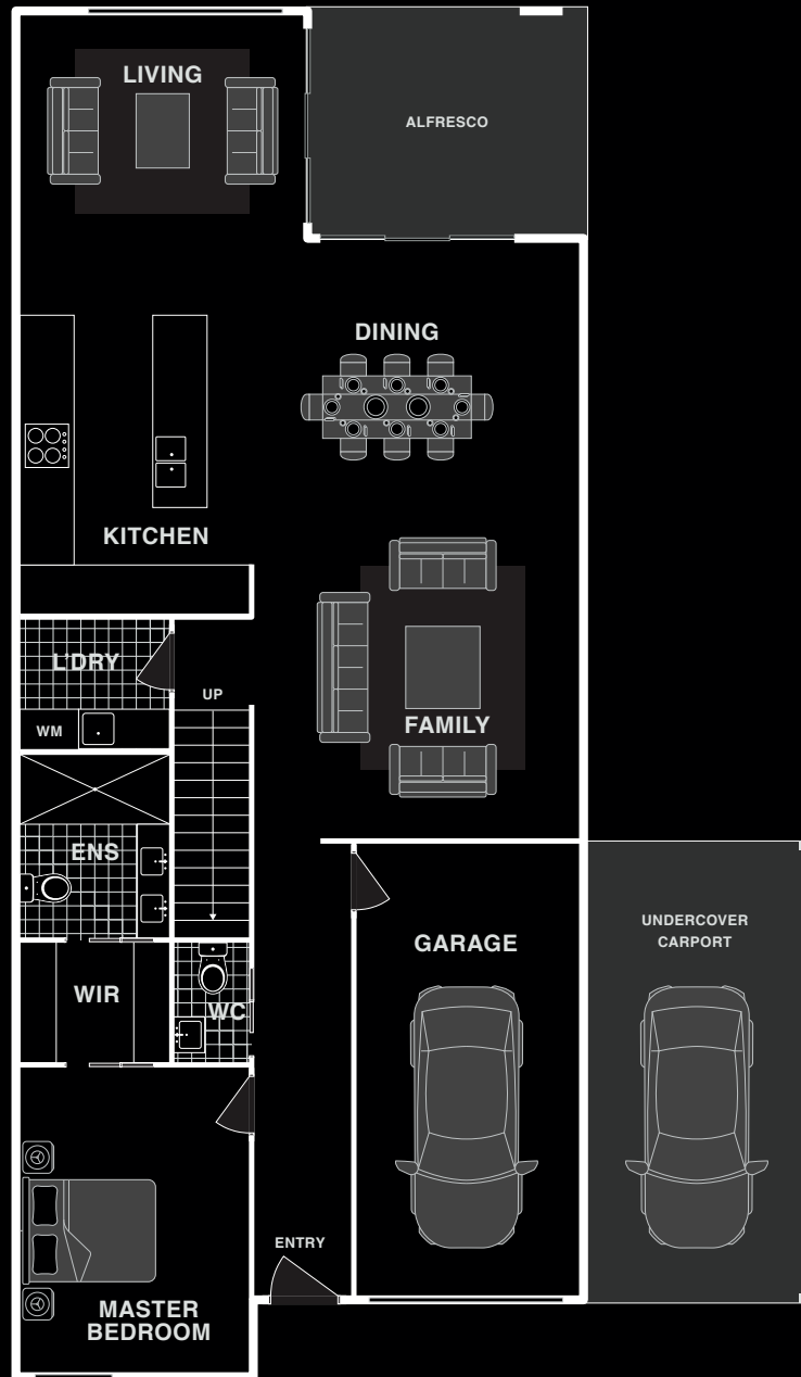
GROUND LEVEL
