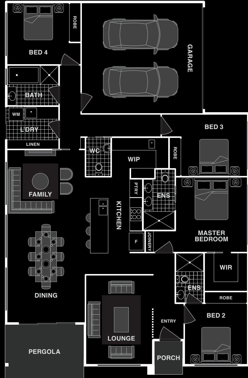
FLOOR PLAN
