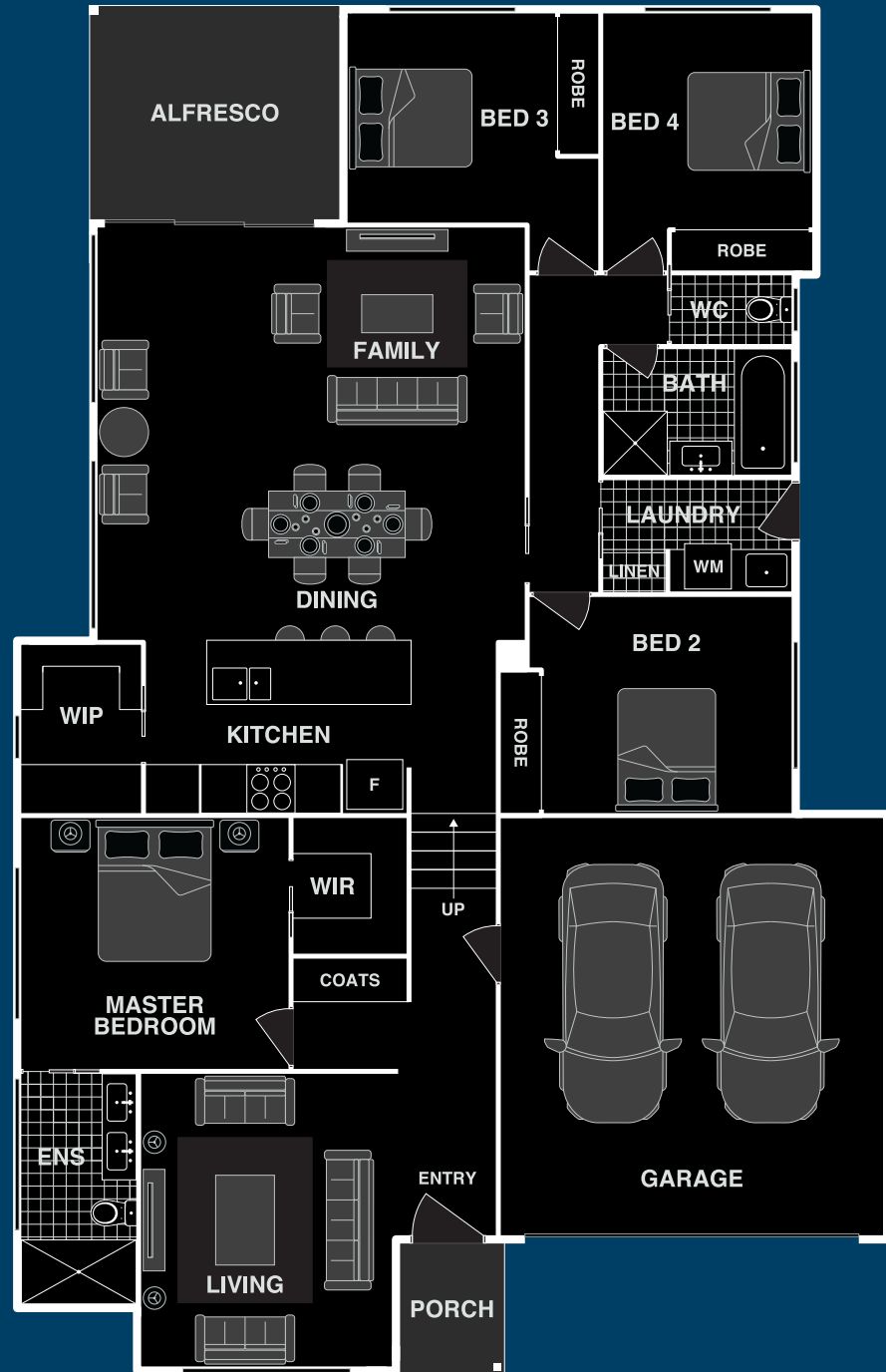
FLOOR PLAN
