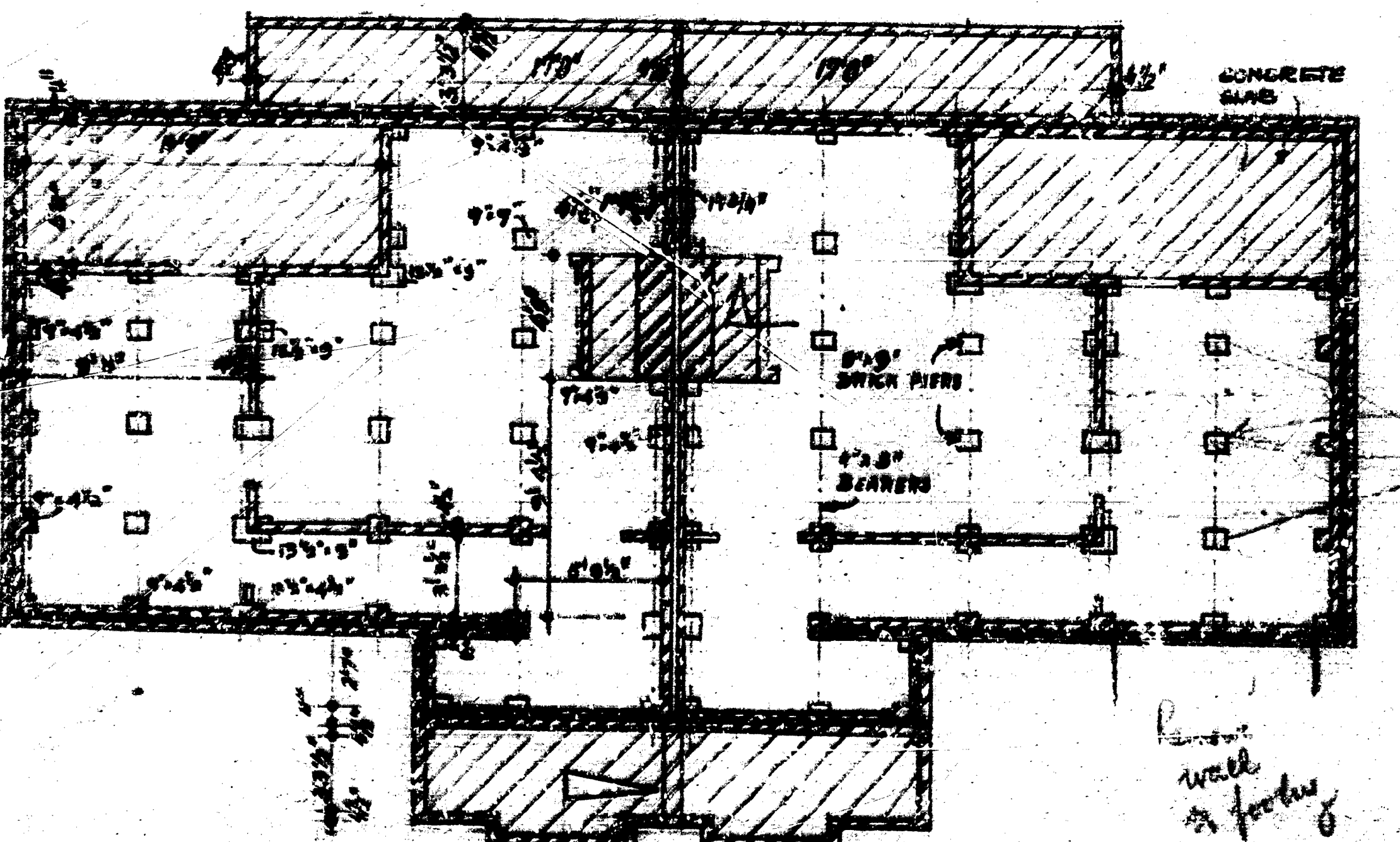
FOUNDATION
