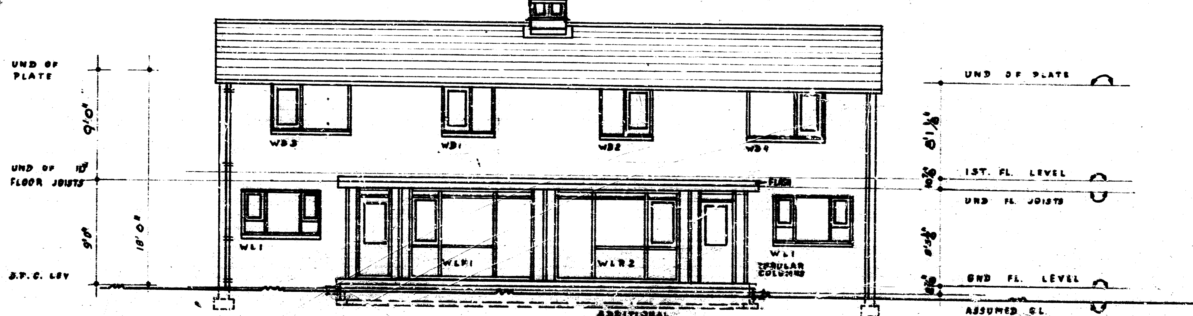
GARDEN ELEVATION
