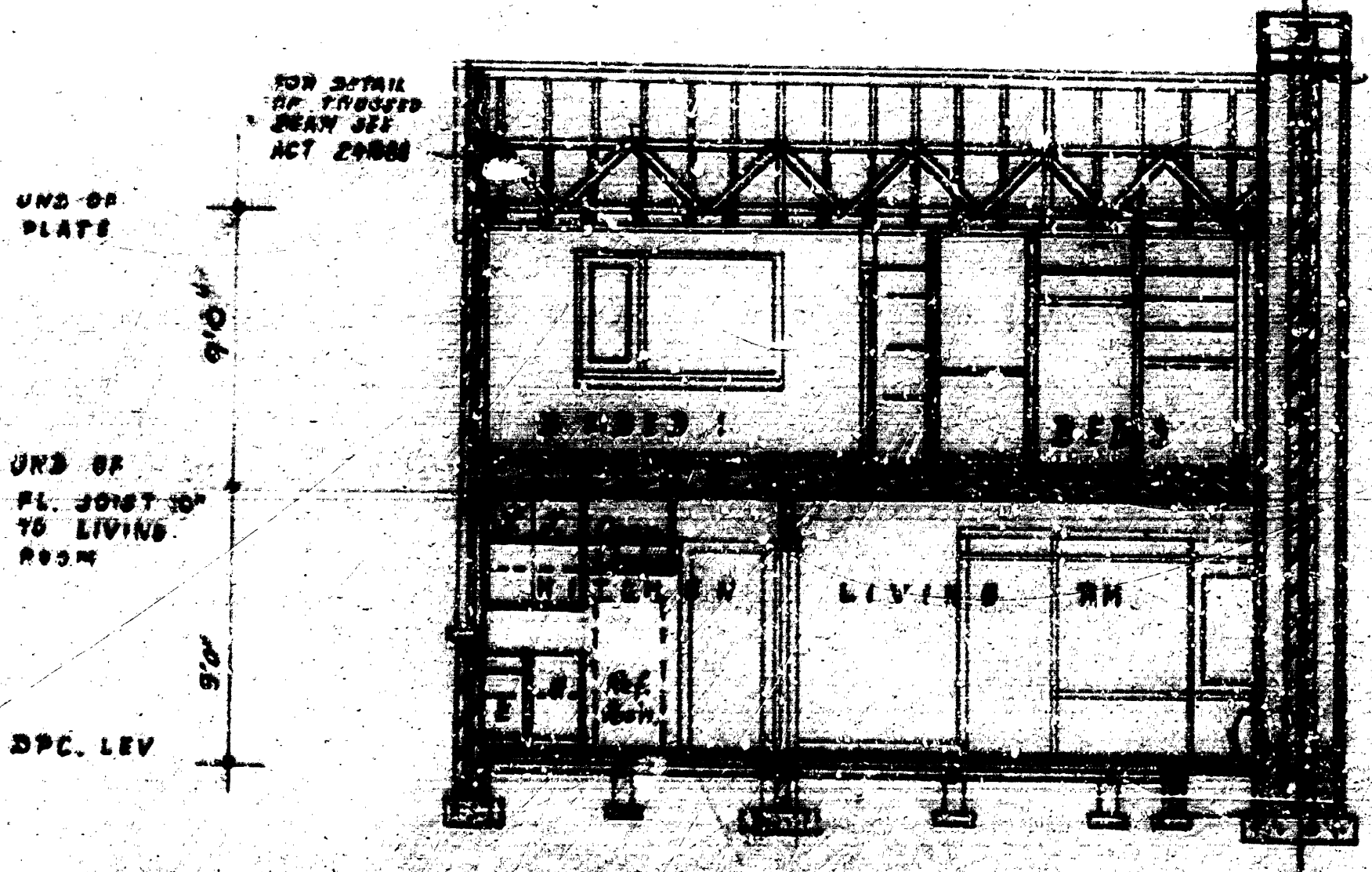
LONG SECTION
