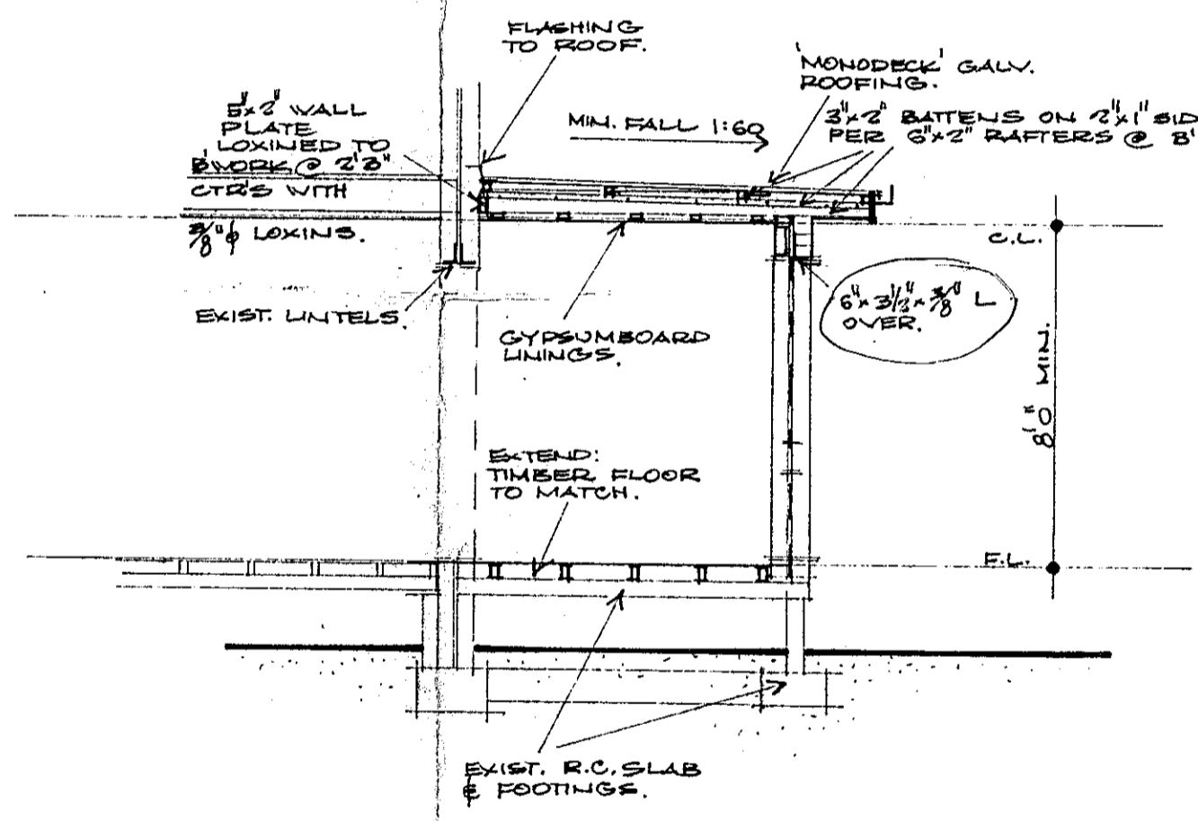
SECTION
