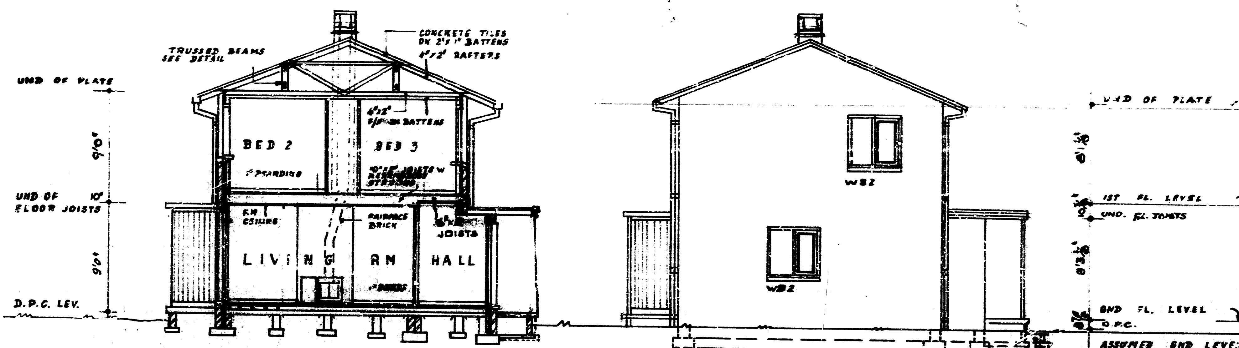
GROSS SECTION
