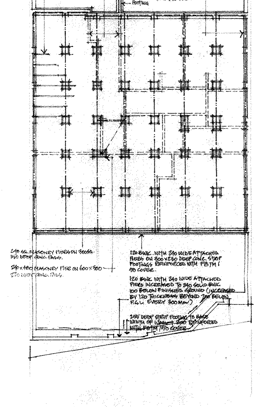
SITE & FOUNDATION PLAN.
