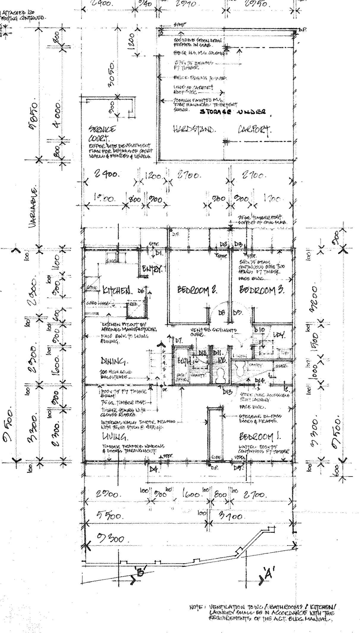
FLOOR PLAN.
