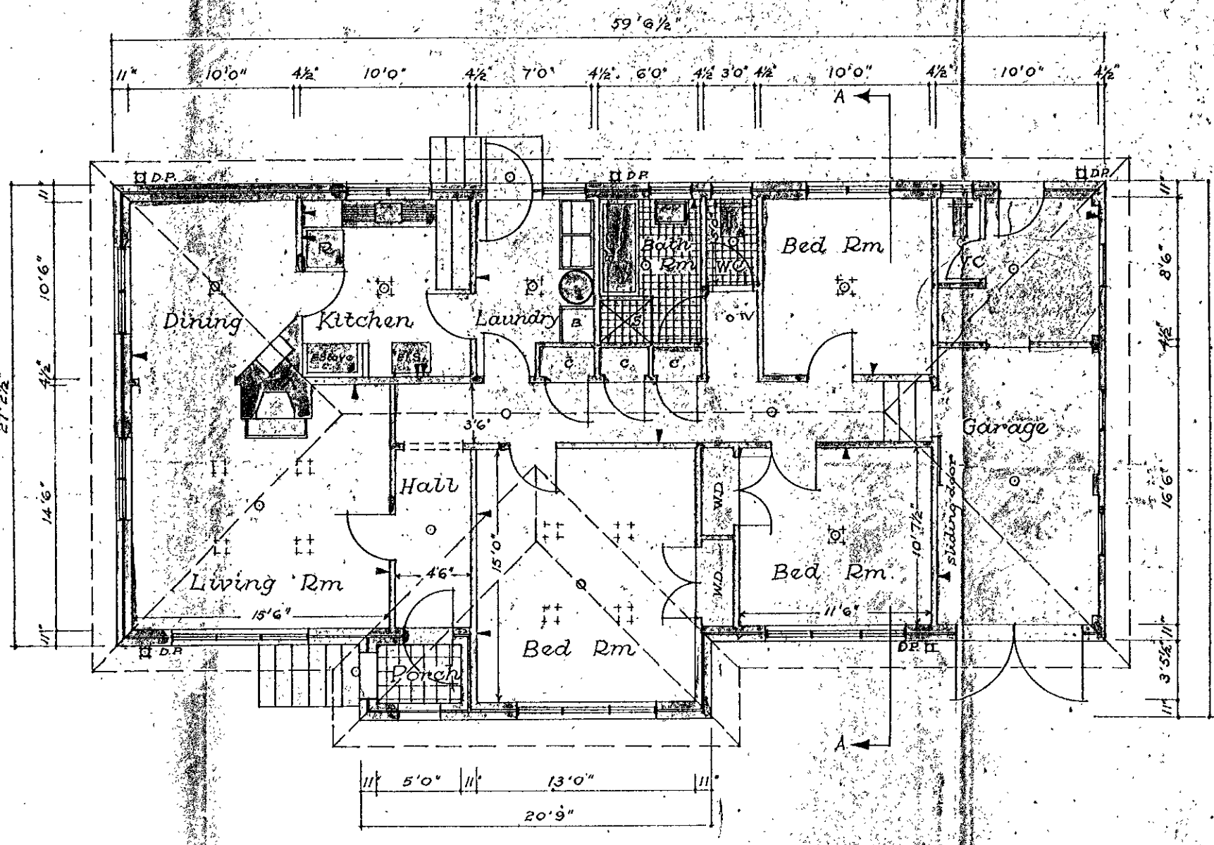
PLAN
