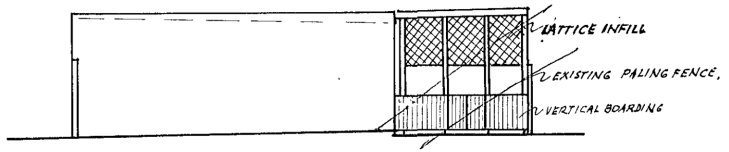
SIDE ELEVATION
