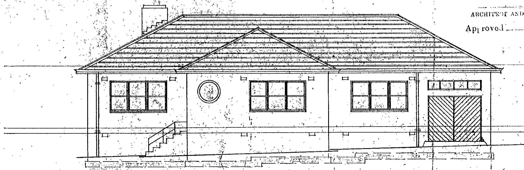
FRONT ELEVATION
