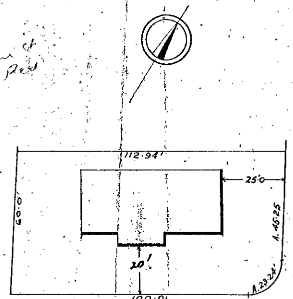
SITE PLAN Scale: 40' = 1"
