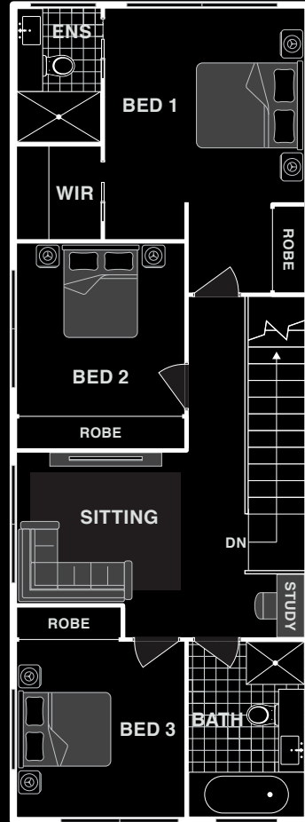
UPPER LEVEL
